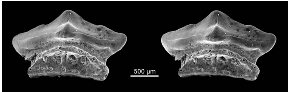
Fig. 6. Lissodus angulatus (Stensiö, 1921) – labial view. ZPAL P.8/1-B21. SEM stereo-micrographs. Vardebukta Formation, Lower Triassic (Dinerian); Hyrnefjellet Mt., Hornsund.
