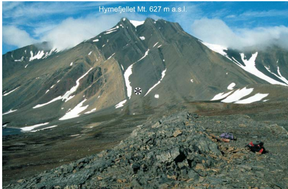
Fig. 2. Outcrops of the late Paleozoic–early Mesozoic sequence. Hyrnefjellet Mt., Hornsund. Asterisk shows shark teeth sampling locality. Photo taken by A. Gaździcki, July 1998.
