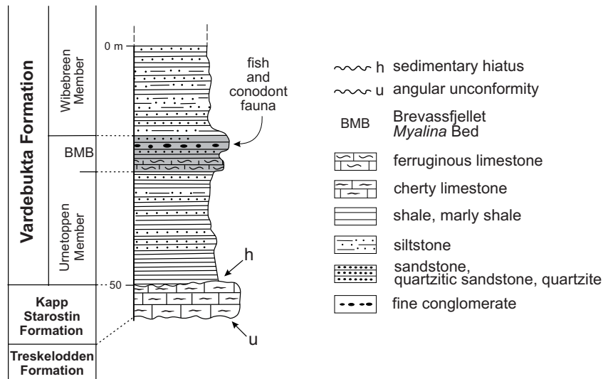
Fig. 3. Position of the fish fauna in the Triassic stratigraphic log of the Hyrnefjellet Mt., Hornsund (after Birkenmajer 1977).
