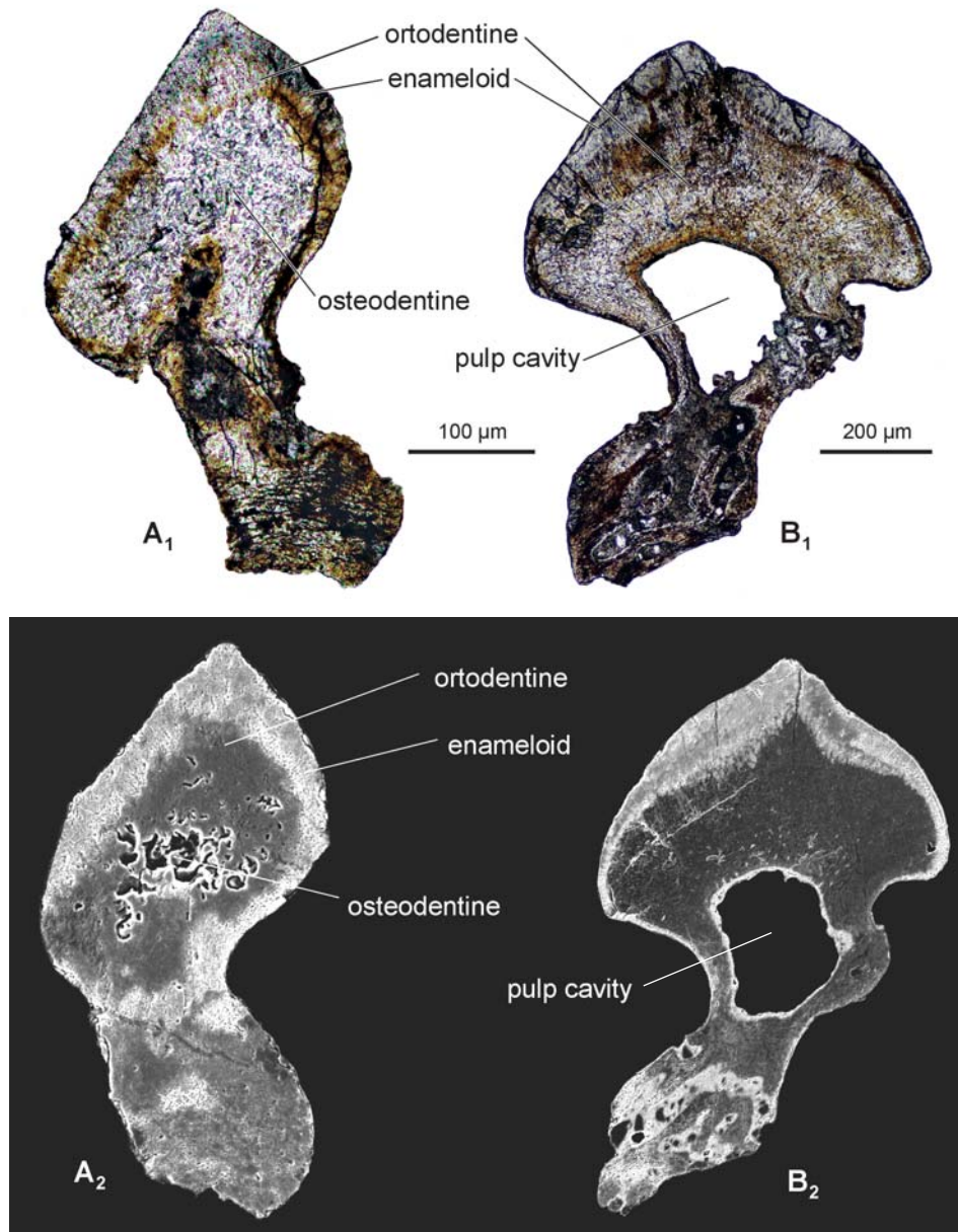
Fig. 10. Vertical sections of Lissodus angulatus (Stensiö, 1921) teeth from the Vardebukta Formation, Lower Triassic (Dinerian), Hymefjellet Mt., Hornsund. A. ZPAL P.8/1-BB1 – posterior tooth. B. ZPAL P.8/1-BB2 – anterior tooth. A 1 –B 1 – thin sections, A 2 –B 2 – SEM micrographs.
