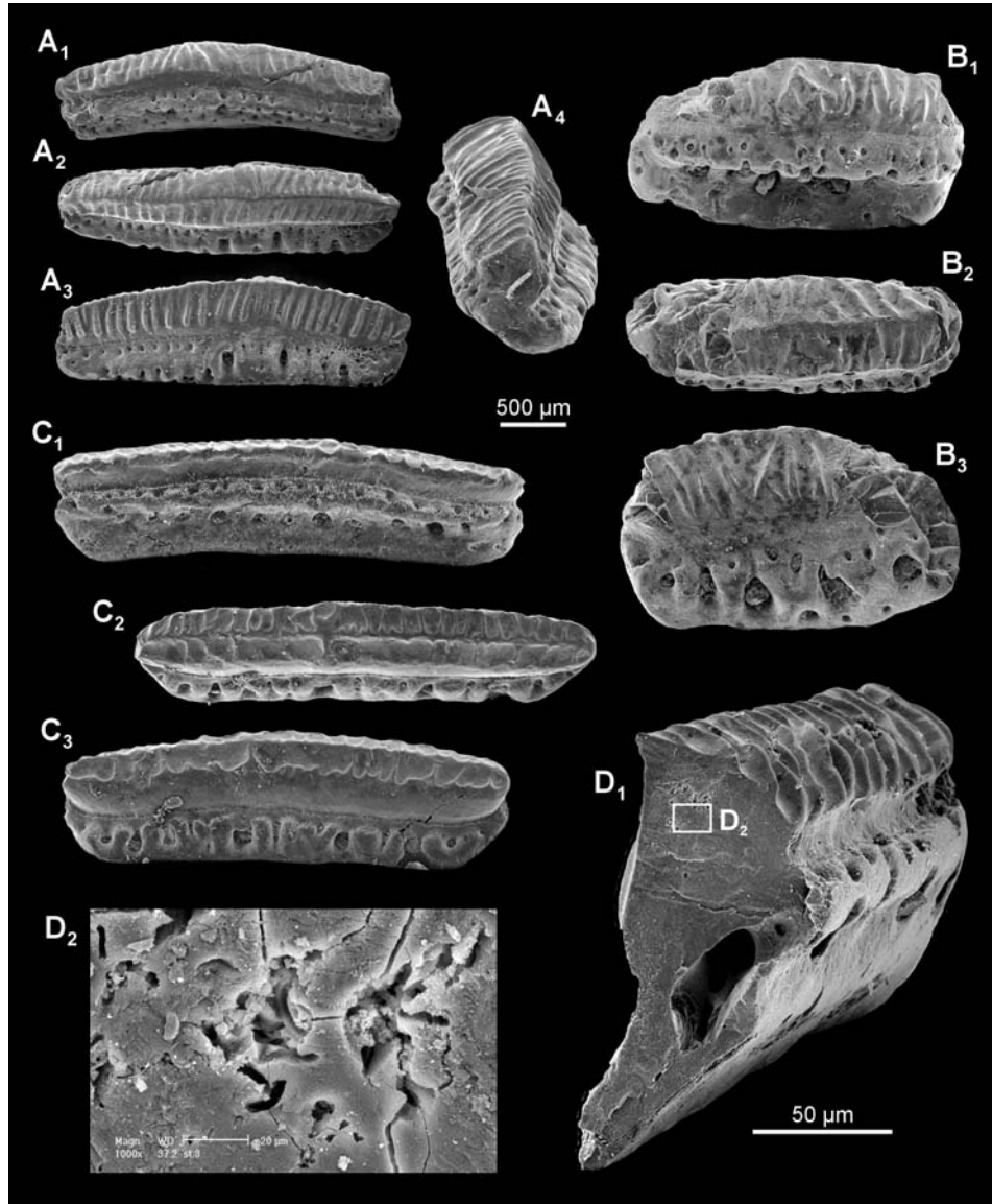
Fig. 8. Teeth of Acrodus spitzbergensis Hulke, 1873. A. ZPAL P.8/2-B45, A 1 – labial view, A 2 – occlusal view, A 3 – lingual view, A 4 – lateral view. B. ZPAL P.8/2-B34, B 1 – labial view, B 2 – occlusal view, B 3 – lingual view. C. ZPAL P.8/2-B15, C 1 – labial view, C 2 – occlusal view, C 3 – lingual view. D. ZPAL P.8/2-B32, D 1 – cross-section, D 2 – osteodentine. Vardebukta Formation, Lower Triassic (Dinerian); Hyrnefjellet Mt., Hornsund.
