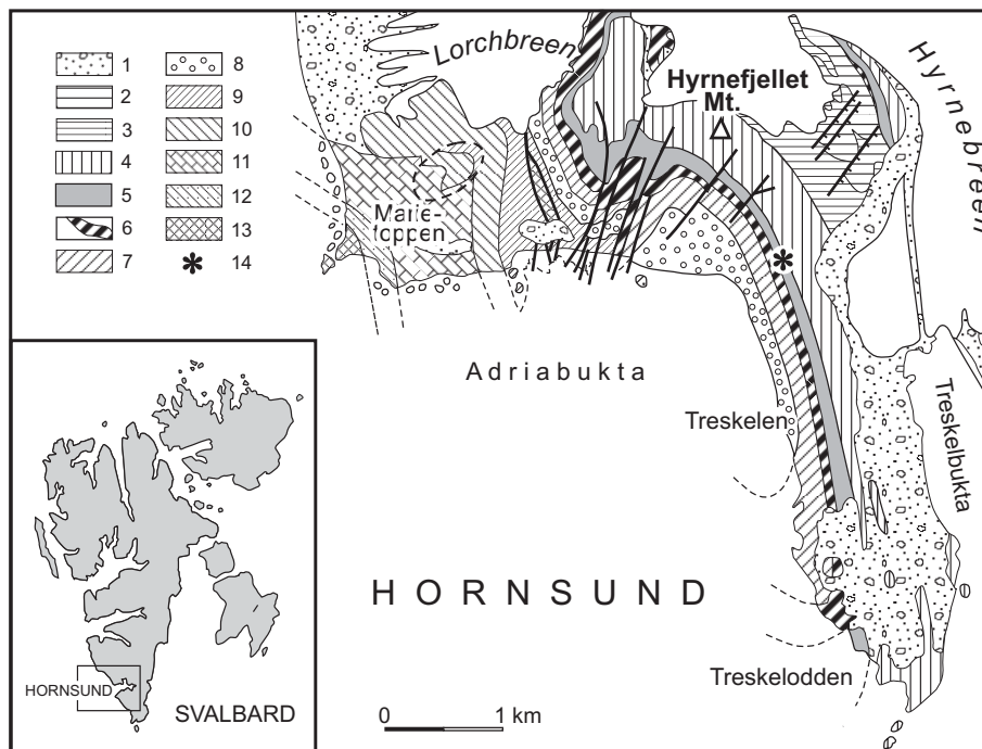
Fig. 1. Geological map of West Spitsbergen (Hornsund area) showing the location of the Hyrnefjellet Mt., where the specimens of shark teeth were collected. 1 – Moraines, partly outwash; 2 – Festningen Sandstone (Hauterivian–Barremian); Ullaberget Series (Lower Neocomian); 3 – Tiolarpasset Series (Volgian–Lower Neocomian); 4 – Middle and Upper Triassic; 5 – Lower Triassic; 6 – Brachiopod Cherty Limestone (Upper Permian); 7 – Treskelødden Beds (Upper Carboniferous–lowermost Permian); 8 – Hyrnefjellet Beds (Middle Carboniferous); 9 – Adriabukta Series (Visean–Namurian A?); 10 – Upper Marietoppen Series (Devonian: Grey Hoek Series?); 11 – Middle Marietoppen Series (Devonian: Stjørdalen Division?); 12 – Lower Marietoppen Series (Devonian: Keltiefjellet Division?); 13 – Sofiebogen Formation (Eocambrian–Precambrian); 14 – Shark teeth sampling locality. After Birkenmajer (1964).
