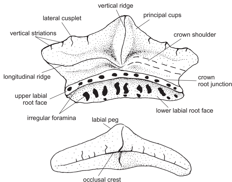
Fig. 5. Descriptive nomenclature of Lissodus tooth modified from Duffin (1985).
