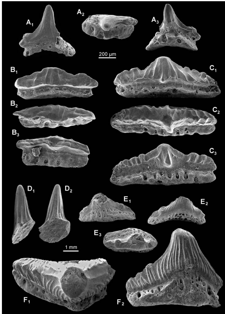
Fig. 9. A–C. Teeth of Hybodus microdus Stensiö, 1921. A. ZPAL P.8/3-B17, A 1 – labial view, A 2 – occlusal view, A 3 – lingual view. B. ZPAL P.8/3-B35, B 1 – labial view, B 2 – occlusal view, B 3 – lingual view. C. ZPAL P.8/3-B14, C 1 – labial view, C 2 – occlusal view, C 3 – lingual view. D. Hybodus sp. ZPAL P.8/4-B11, D 1 – lateral view, D 2 – lingual view. E–F. Hybodus sasseniensis Stensiö, 1918. E. ZPAL P.8/4-B51, E 1 – lingual view, E 2 – labial view, E 3 – occlusal view. F. ZPAL P.8/4-B52, F 1 – occlusal view, F 2 – lingual view. Vardebukta Formation, Lower Triassic (Dinerian); Hymefjellet Mt., Hornsund.
