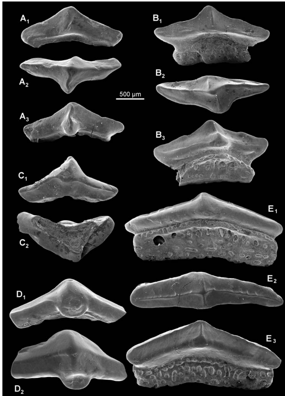
Fig. 7. Teeth of Lissodus angulatus (Stensiö, 1921). A. ZPAL P.8/1-B25, A 1 – lingual view, A 2 – occlusal view, A 3 – labial view. B. ZPAL P.8/1-B21, B 1 – lingual view, B 2 – occlusal view, B 3 – labial view. C. ZPAL P.8/1-B48, C 1 – occlusal view, C 2 – basal view. D. ZPAL P.8/B210, D 1 – lingual view, D 2 – occlusal view. E. ZPAL P.8/1-B22, E 1 – lingual view, E 2 – occlusal view, E 3 – labial view. Vardebukta Formation, Lower Triassic (Dinerian); Hyrnefjellet Mt., Hornsund.
