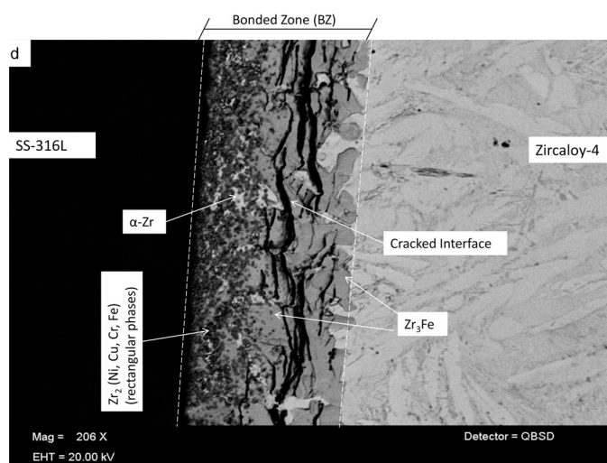
Fig. 2d. Back-scattered image (BSI) showing different phases and crack in BZ
