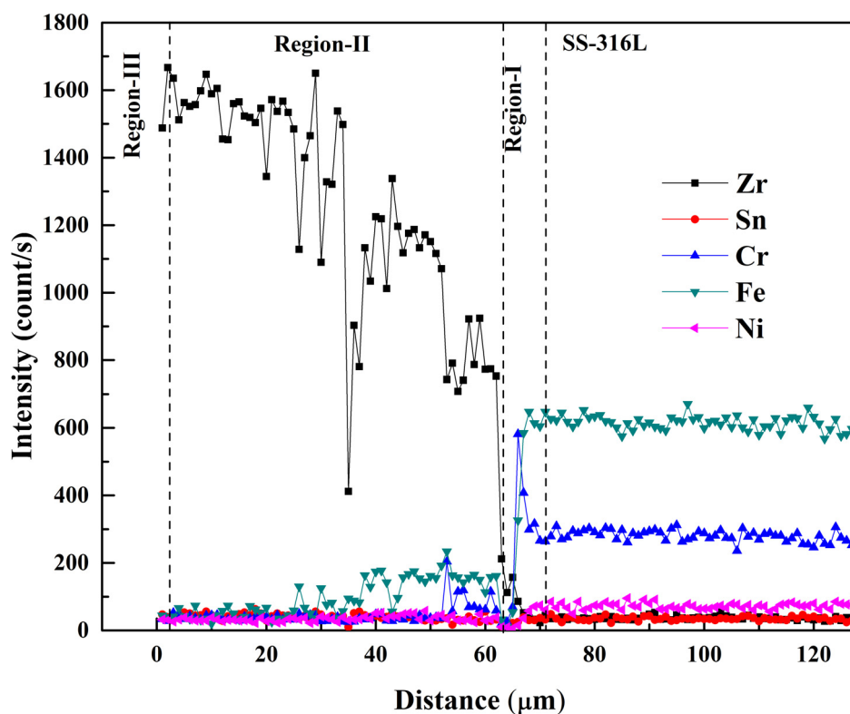
Fig. 3. The compositional line scan of BZ through EDS
