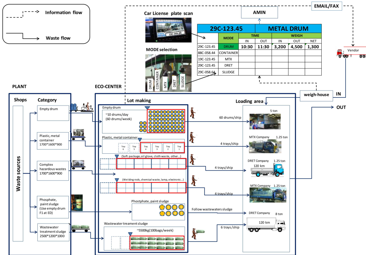
Fig. 7. Truck calling system using Andon (Example for hazardous waste).
