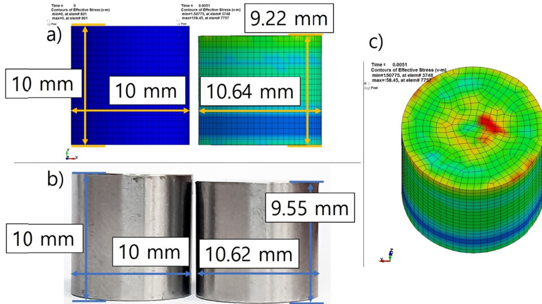
Fig. 1. Numerical (a) and experimental (b) result of high speed deformation and residual stress generation. And top surface of numerical analysis result (c)
