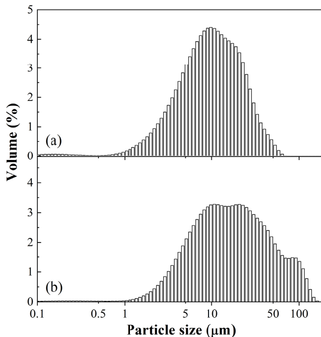
Fig. 2. Particle size distribution of the ball-milled powders with 1 wt% of (a) stearic acid and (b) ethanol as PCA
