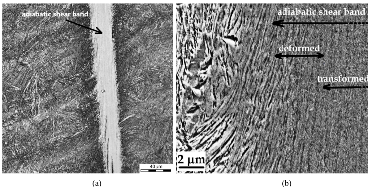
Fig. 11. Microstructure within the area of adiabatic shear band. Nanostructured bainitic steel: variant B-210 – punch velocity of 797 mm/s; punch displacement of 0.55 mm; (a) light microscope; (b) scanning electron microscope
