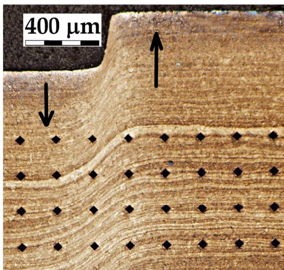
Fig. 9. Macrostructure and hardness distribution within the shear zone without ASB. Nanostructured bainitic steel – variant B-210; punch velocity of 0.3 mm/s; punch displacement of 0.3 mm
