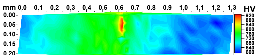
Fig. 10. Macrostructure and hardness distribution within the shear zone with ASB. Nanostructured bainitic steel: variant B-210; punch velocity of 30.4 mm/s; punch displacement of about 0.85 mm
