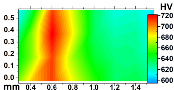
Fig. 9. Macrostructure and hardness distribution within the shear zone without ASB. Nanostructured bainitic steel – variant B-210; punch velocity of 0.3 mm/s; punch displacement of 0.3 mm
