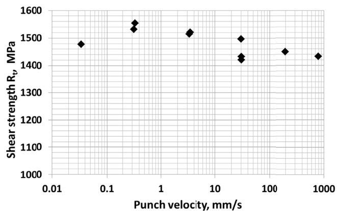
Fig. 8. Shear strength vs. punch velocity in the range up to 800 mm/s. Nanostructured bainitic steel B-210
