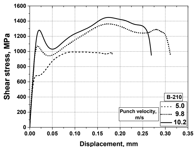
Fig. 13. Dynamic shear stress vs. punch displacement. Nanostructured bainitic steel
