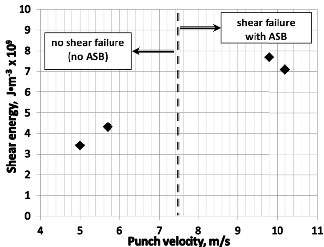
Fig. 18. Shear energy vs. punch velocity, (a) related to volume of shear zone resulted from the difference between diameter of the punch and die; (SHPB experiments)
