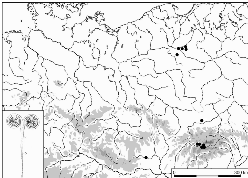
Fig. 7. Distribution of pins with the head in the form of two spirals and with flattened shaft in the Hallstatt period (after Durczewski 1948; Durczewski 1961; Kostrzewski 1964; Novotná 1970, Říhovský 1979, Rydzewski 1995)
