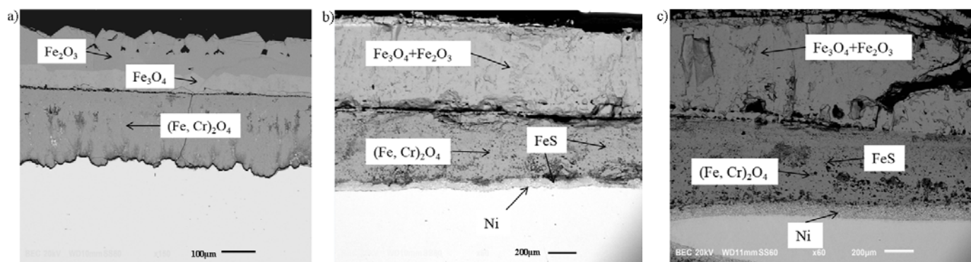
Fig. 7. SEM cross sections of scales. a – CO 2 (900°C), b – CO 2 +1 vol.% SO 2 (900°C), c – CO 2 +5 vol.% SO 2 (900°C)
