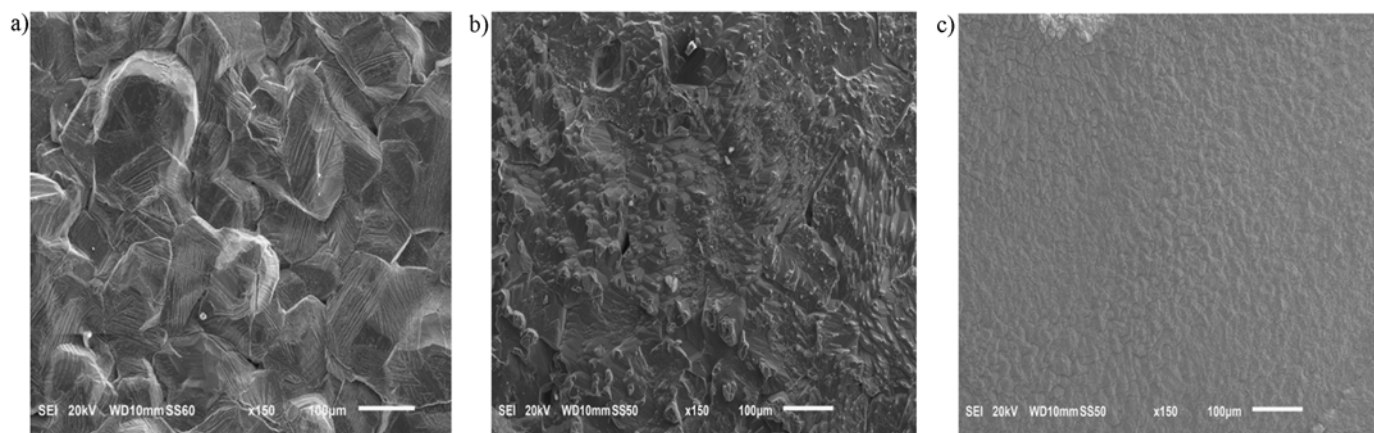
Fig. 6. Morphology (SEM) of scales surface. a – CO 2 (900°C), b – CO 2 +1 vol.% SO 2 (900°C), c – CO 2 +5 vol.% SO 2 (900°C)
