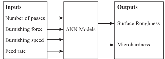
Fig. 4. ANN functional representation of input/output data
