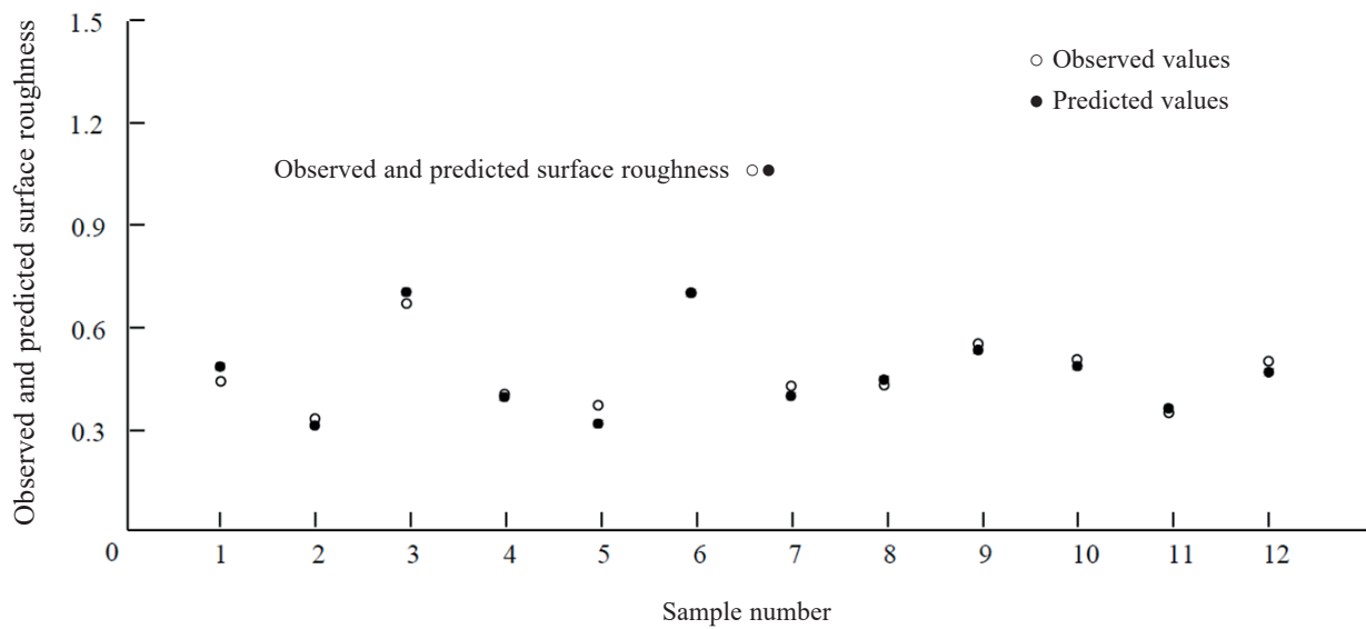
Fig. 7. Relation of the predicted values to the obtained surface roughness values
