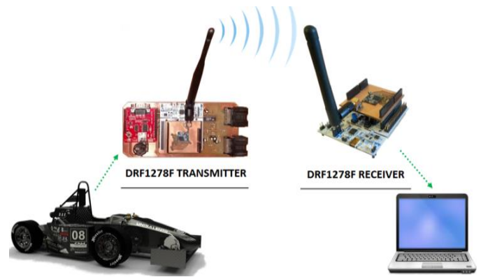
Fig. 4. Base station on the right with DRF1278F radio module in reception mode connected with PC through a ST Nucleo board and realized telemetry system on the left inside the car for data sensors detection and transmission.
