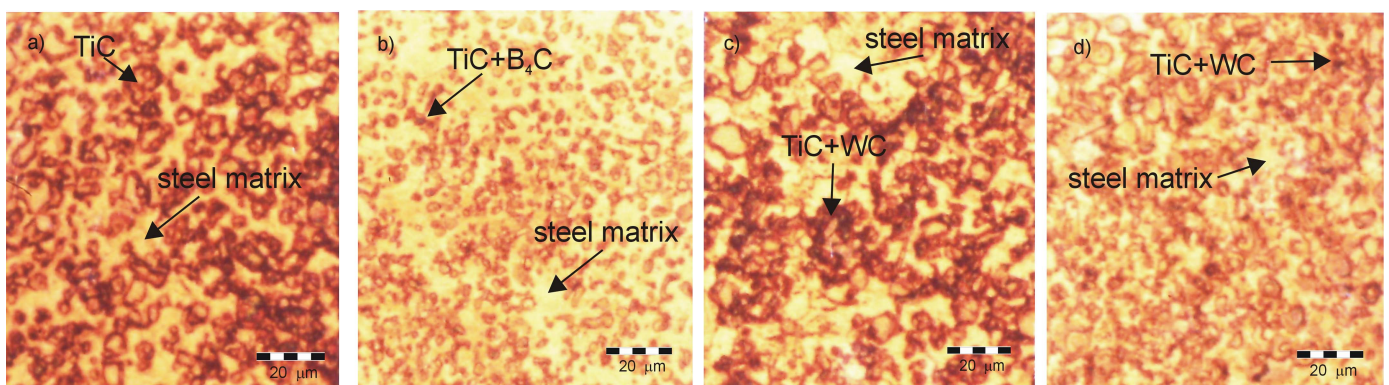
Fig. 13. Microstructure of Ferro-TiC CM composite: a) unmodified, b) with 11.9 vol. % B_4C and c) with 2.1 vol. % WC, d) with 11.2 vol.% of WC; sintering at 1360°C for 40 minutes
