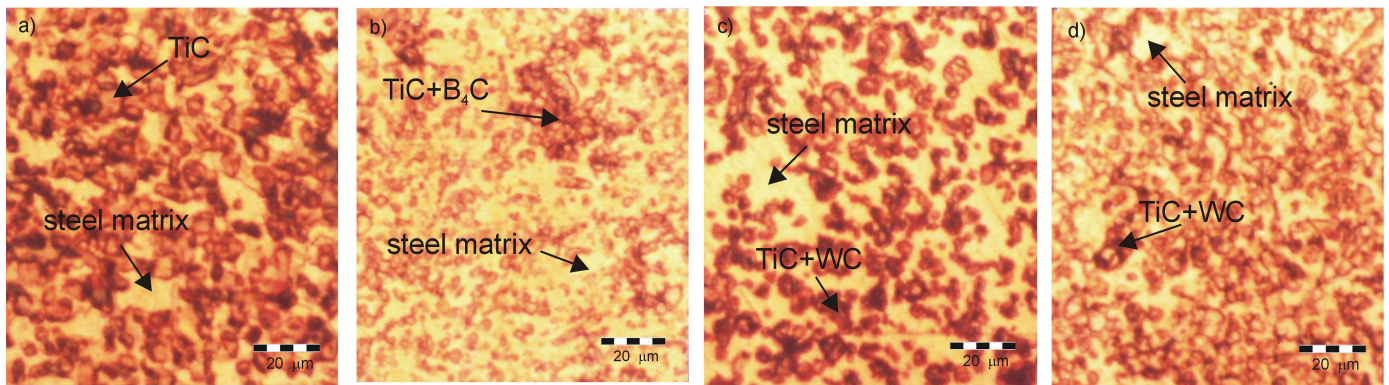
Fig. 12. Microstructure of Ferro-TiC CM composite: a) unmodified, b) with 11.9 vol. % B_4C and c) with 2.1 vol.% WC, d) with 11.2 vol.% of WC; sintering at 1380°C for 40 minutes
