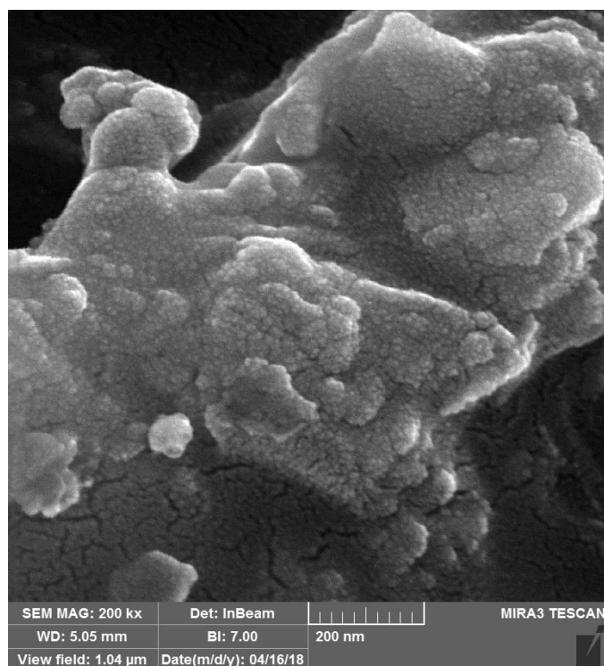
Fig. 2. SEM image of the synthesized chalcopyrite \text{CuFeS}_2
