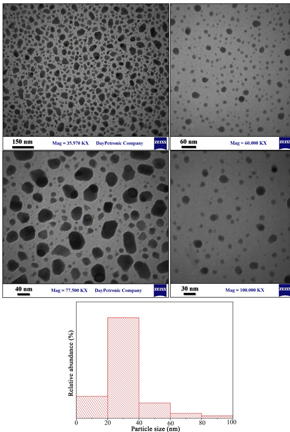
Fig. 3. TEM image and particle size histogram of the synthesized chalcopyrite \text{CuFeS}_2
