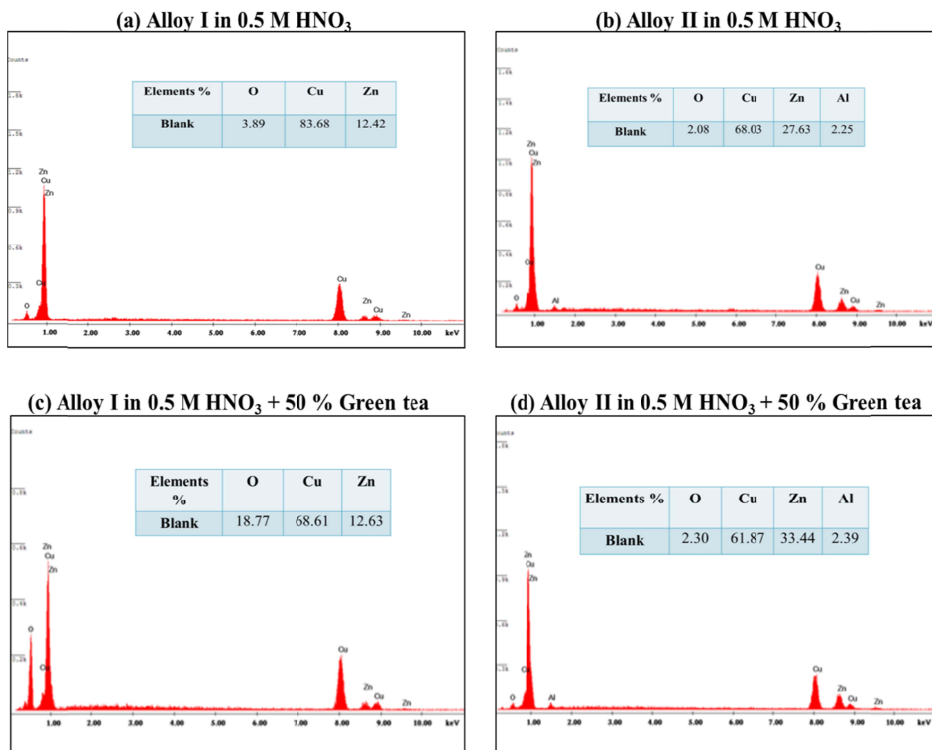
Fig. 11. EDX spectra and percentage of elements present on Cu-Zn alloys in 0.5 M \text{HNO}_3 solution in the absence and presence of 50% green tea
