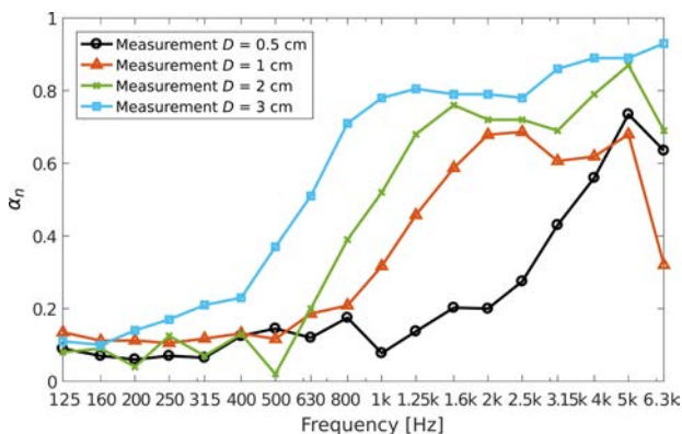
Fig. 6. Sound absorption coefficient comparisons for D = 0.5 cm, D = 1 cm, D = 2 cm, D = 3 cm.
