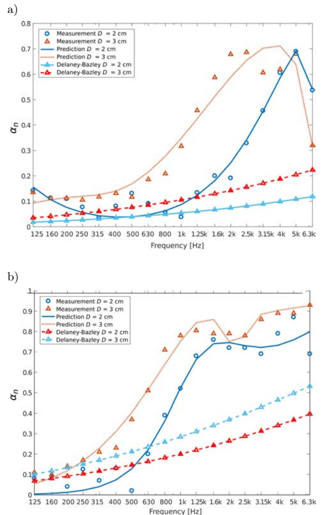
Fig. 7. Sound absorption coefficient of 23.15 kN/m 2 absorber with different thickness: a) sample 1A and 1B; b) sample 2 and sample 3.
