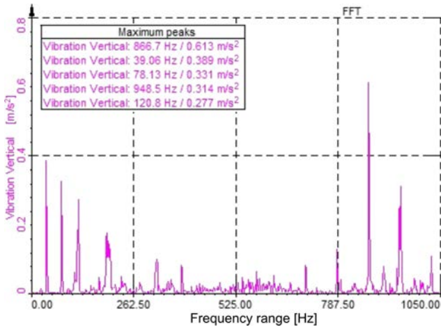
Fig. 3. Spectral view of vibration frequencies (radial direction).
