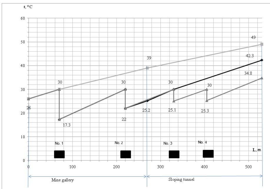
Fig. 2. The change in temperature oil gallery:
