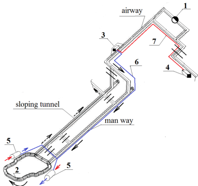
Fig. 3. The scheme of arrangement of underground water-cooling refrigerating machines with a capacity of 500 kW into the mine: 1 – shaft trunk; 2 – mine gallery; 3 – refrigerating machine; 4 – water cooler; 5 – air cooler; 6 – supply pipeline; 7 – return pipeline; —> – fresh air; - - > – return air
