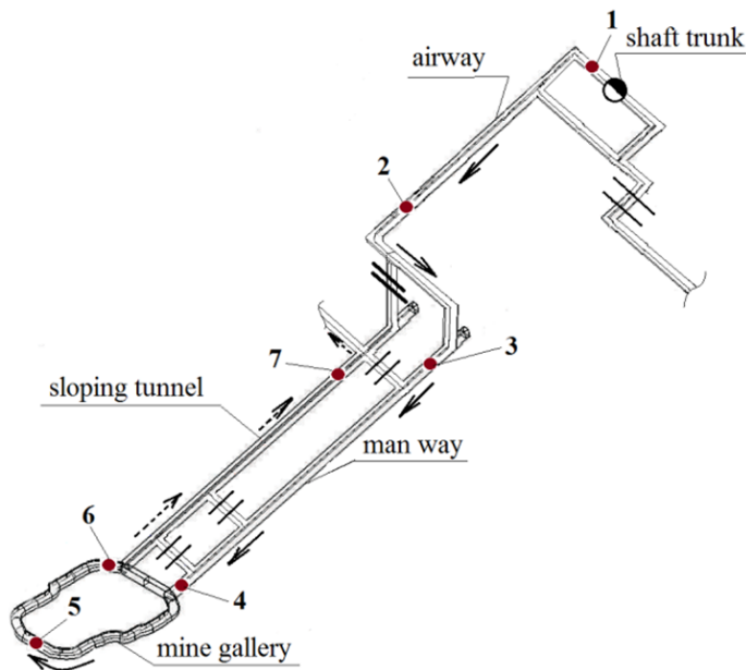
Fig. 1. The scheme of location of points of measurements along the route of the oil gallery: 1-7 – point of measurement hydrothermal characteristics, —> – fresh air, - - > – return air
