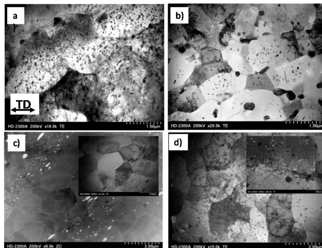
Fig. 4. STEM microstructure of Al-5Cu alloy after KoBo processing. Reduction coefficient \lambda = 30 (a,b) and \lambda = 98 (c,d)
