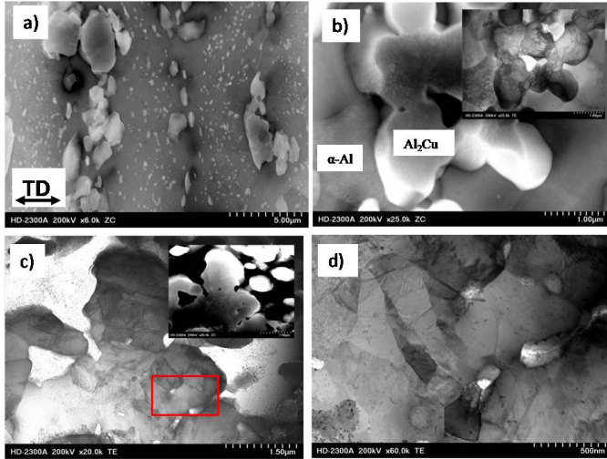
Fig. 6. STEM microstructure of Al-25Cu alloy after KoBo processing. Reduction coefficient \lambda = 30 (a,b) and \lambda = 98 (c,d). Fig. d) is the enlarged area marked with a red square on Fig. c)
