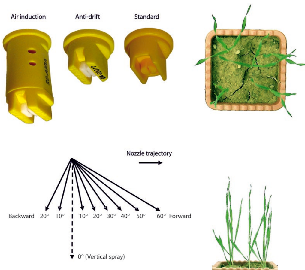
Fig. 1. Wild barley having vertically-oriented leaves at herbicide application time, the nozzles used in the study, and the angling of their spray from 20^\circ backward to 60^\circ forward relative to the direction of nozzle trajectory
