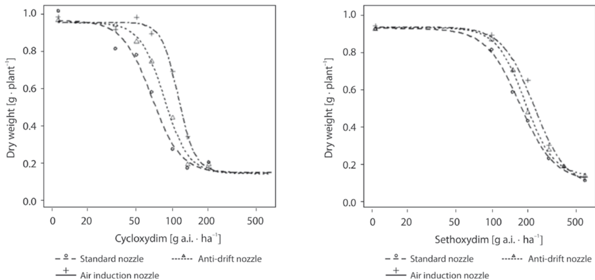
Fig. 2. Response of wild barley dry weight to doses of cycloxydim and sethoxydim sprayed vertically using standard ( \circ ), anti-drift ( \Delta ) and air induction (+) flat fan nozzles. Data points are means of eight replicates from two experiments
