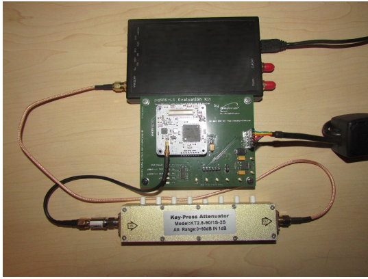
Fig. 13. piNAV receiver test setup.
