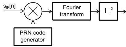
Fig. 7. Block diagram of the parallel Doppler frequency search algorithm.
