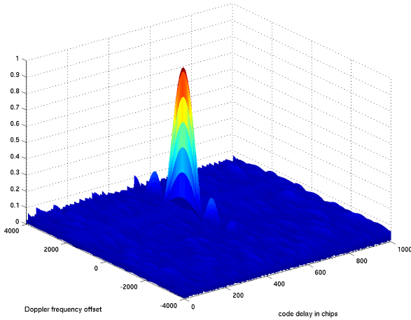
Fig. 1. Two-dimensional correlation function of GPS L1 signal.
