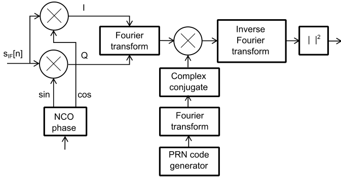
Fig. 8. Block diagram of the parallel code phase search algorithm.
