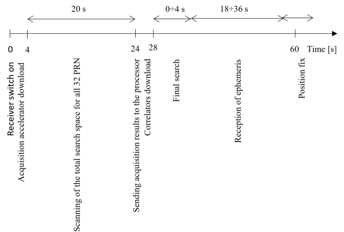
Fig. 12. Cold start time sequence.
