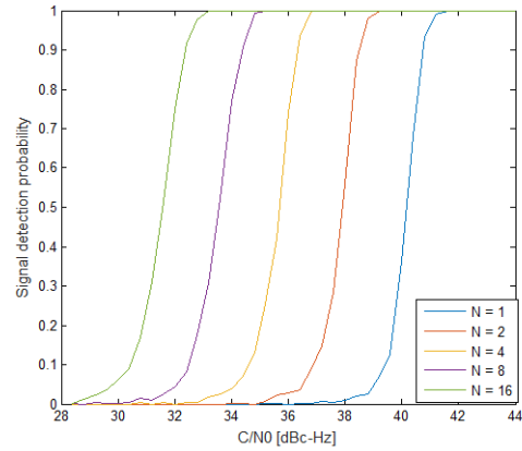
Fig. 4. Probability of detection for GPS L1 signal, T_I=1 ms, N_c=128000 cells.
