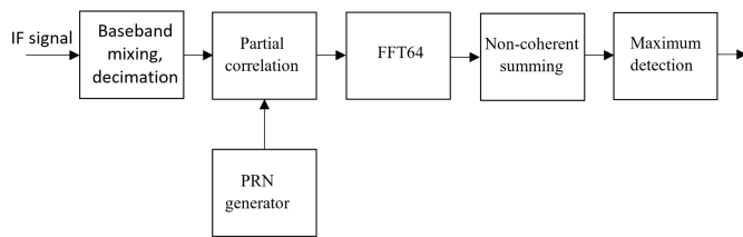
Fig. 11. Acquisition accelerator block scheme.
