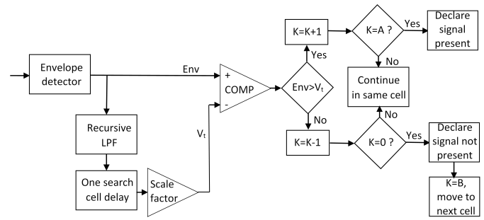
Fig. 5. Tong algorithm flowchart.
