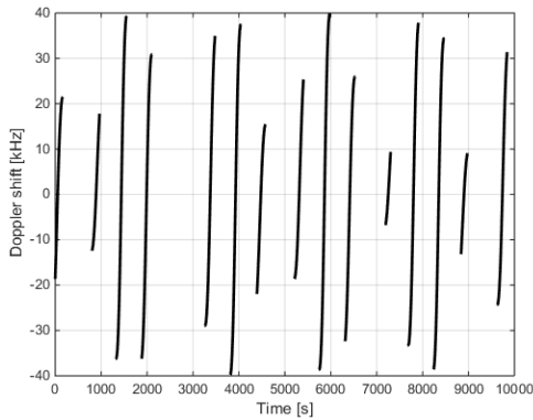
Fig. 2. Doppler shift of GPS L1 signal measured on LEO orbit.
