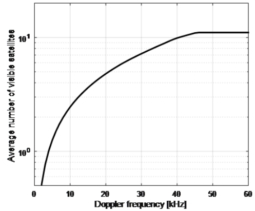
Fig. 3. Average number of visible satellites that have Doppler frequency shift not exceeding given value.
