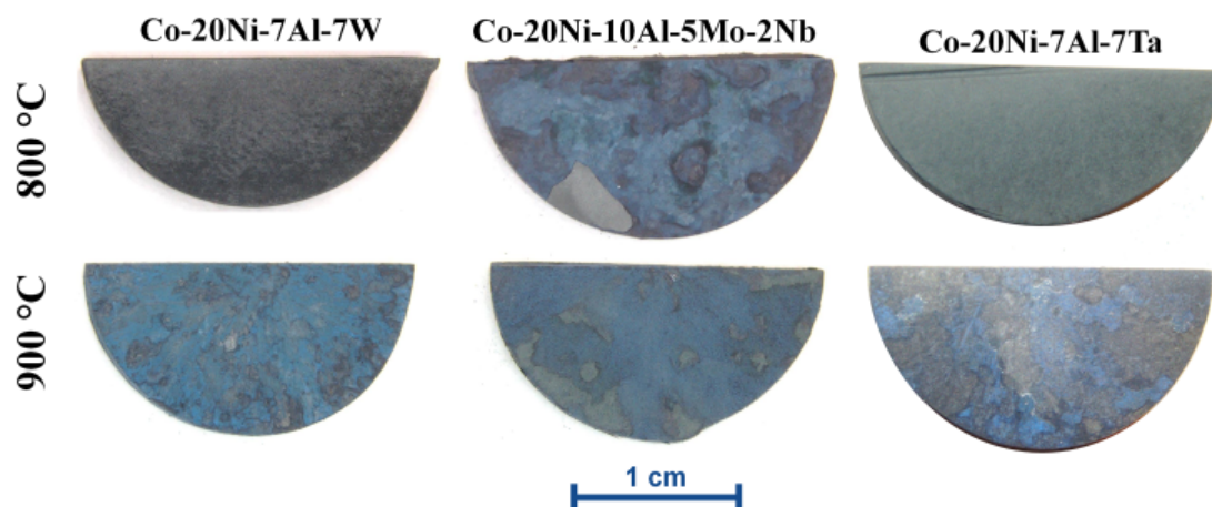
Fig. 2. Macrographs of specimens after oxidation at 800 and 900°C
