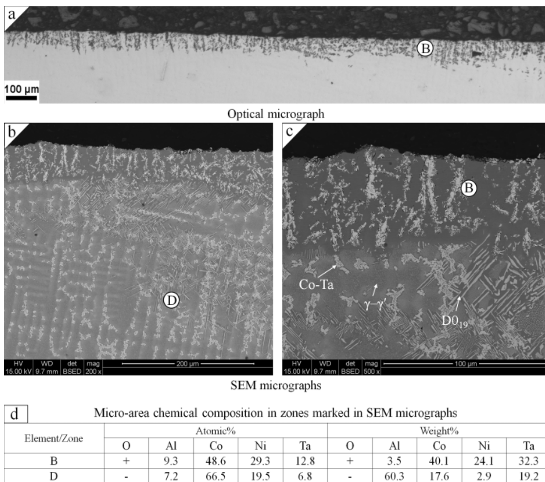
Fig. 12. Cross-sectional micrographs of the scale grown on Co-20Ni-7Al-7Ta alloy after oxidation at 900°C: a) LM micrograph; b and c) SEM micrographs; d) EDS analysis
