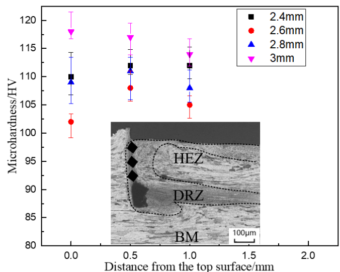
Fig. 7. Microhardness distributions in the sleeve retreating paths of joints under different plunge depths
