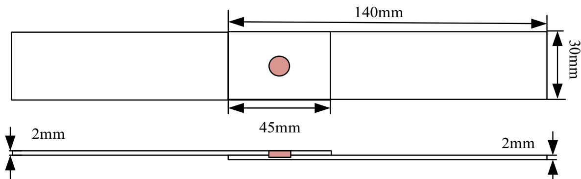
Fig. 1. Schematic of the lap-shear specimen
