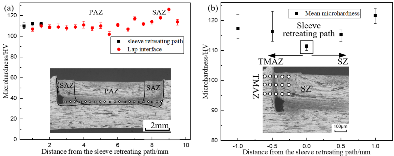
Fig. 8. Microhardness distributions of different regions in RFSSW joint under plunge depth of 2.8 mm: (a) the sleeve retreating path and the lap interface and (b) regions from TMAZ to SZ
