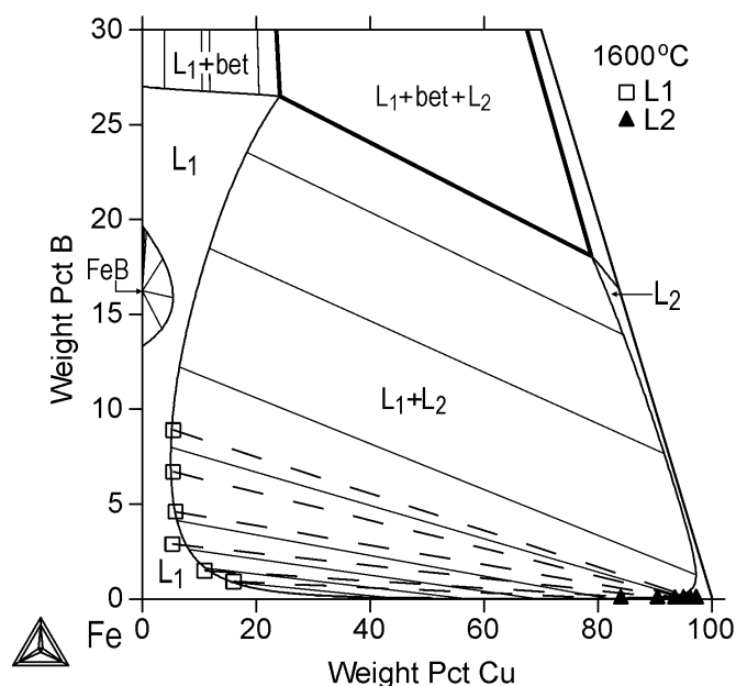
Fig. 8. The calculated isotherm of 1,600°C in the Fe-B-Cu system, with experimental data points of Ono et al. [29]
