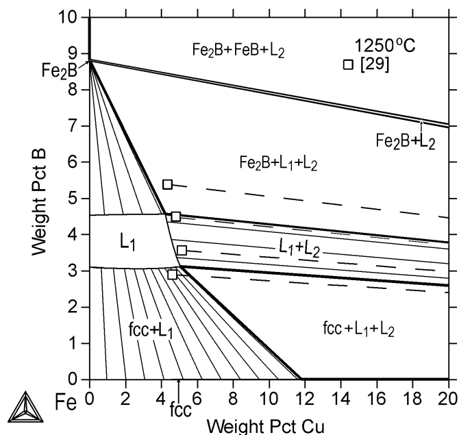
Fig. 10. The calculated isotherm of 1,250°C in the Fe-rich corner of the Fe-B-Cu system, with experimental data points of Ono et al. [29]
