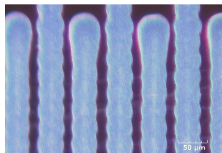
Fig. 12. Widening that occurs at the beginning of thin silver traces. The traces were printed with Sicrys I30EG-1 ink on Kapton substrate
