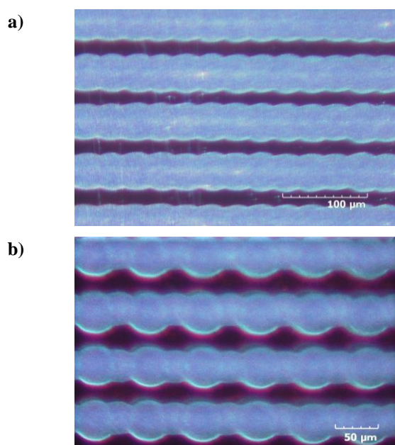
Fig. 11. One-pixel silver traces printed with Sicrys I30EG-1 ink on Kapton substrate. Print was made by two methods: a) vertical orientation print b) horizontal print with splitting the printout into two stages. In both cases, the printhead was shifting horizontally
