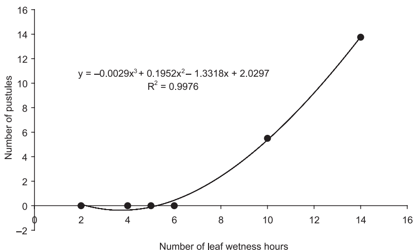
Fig. 1. Effect of leaf wetness period of winter wheat seedlings cv. Micon on the number of Puccinia recondita f. sp. tritici pustules in 15°C
