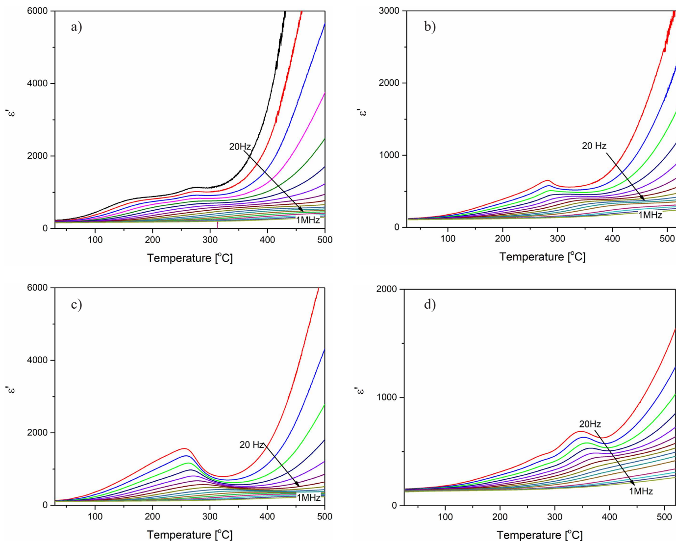
Fig. 6. Temperature dependences of dielectric permittivity for several frequencies chosen for a) BNTF3; b) BNTF5; c) BNTF7; d) BNTF10 ceramics
