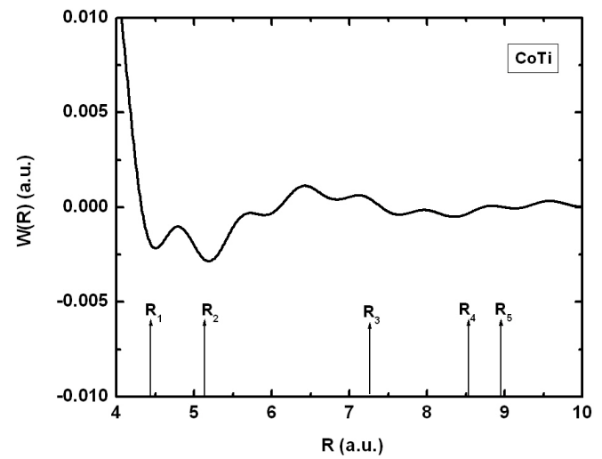
Fig. 1. The dependence of ordering energy on radial distance for CoTi alloy (1 a.u. of energy = 27.2 eV and 1 a.u. of length = 0.529 Å)
