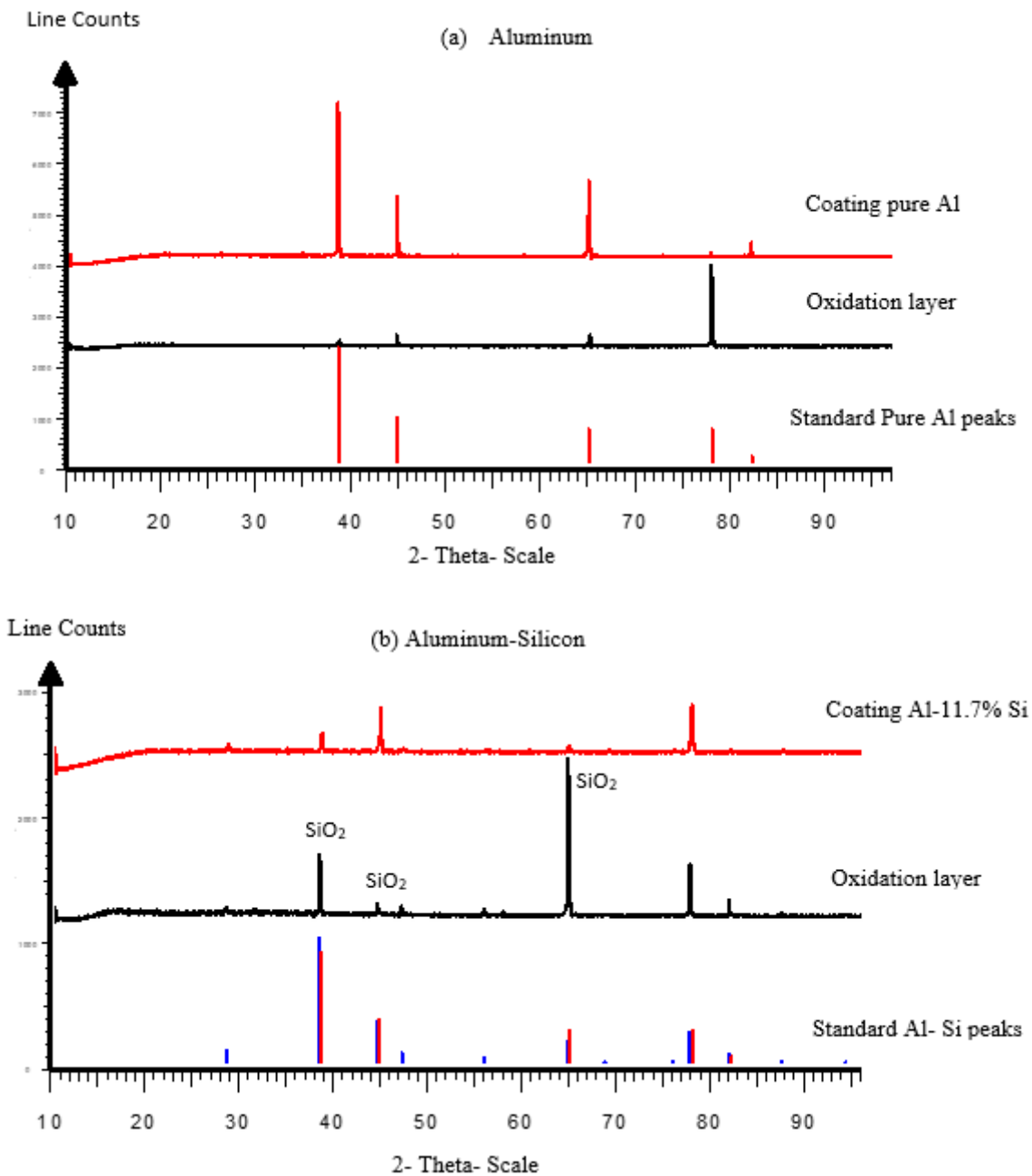
Fig. 8. XRD X- Ray Diffraction pattern after cyclic oxidation of coated samples at 500 °C for 72 hours
