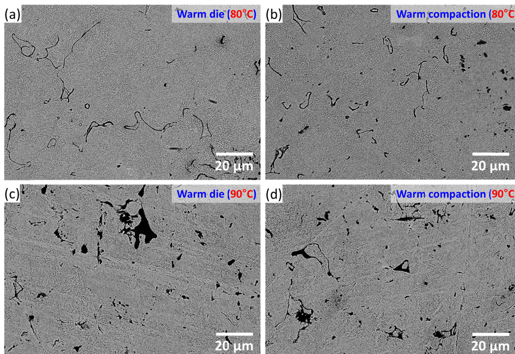
Fig. 4. SEM microstructure of sintered iron mixed with EZ 73 lubricant according to compaction methods and temperatures: (a) warm die at 80°C, (b) warm compaction at 80°C, (c) warm die at 90°C, and (d) warm compacting at 90°C
