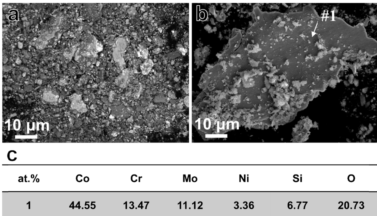
Fig. 4. SEM micrographs showing the wear debris of (a) laser clad WC/T-800 cermet coating layer and (b) bulk T-800 material
