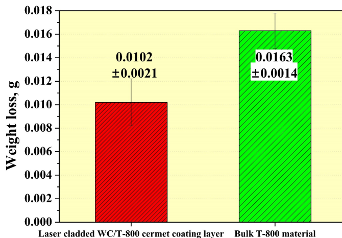
Fig. 2. Pin on disk wear properties of laser clad WC/T-800 cermet coating layer and bulk T-800 material
