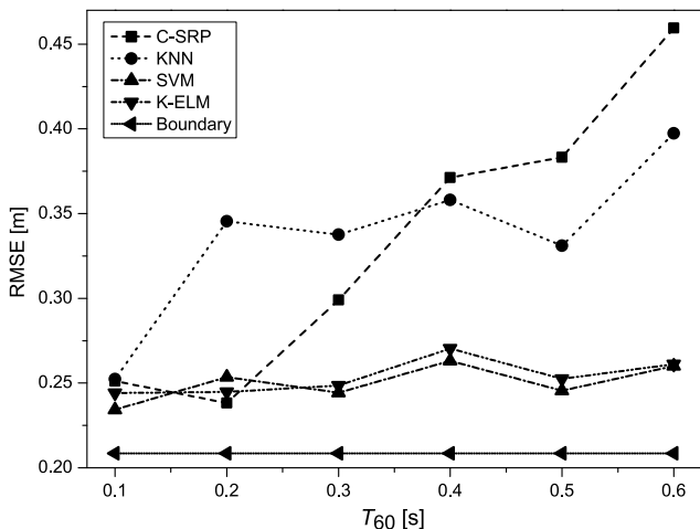
Fig. 5. RMSE of different methods for different T_{60} s with SNR = 15 dB and M = 315 .
