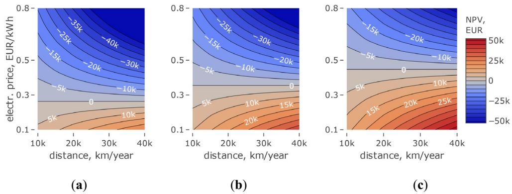
Fig. 2. The NPV as a function of electricity price and yearly distance and for: (a) fuel price = EUR 1 /dm 3 ; (b) fuel price = EUR 1.25 /dm 3 ; (c) fuel price = EUR 1.5 /dm 3 . I_0 = 0 EUR
