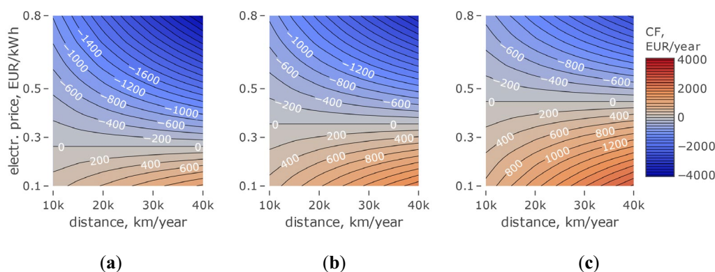
Fig. 1. The Yearly Cash Flow as a function of electricity price and yearly distance and for: (a) fuel price = EUR 1 / \text{dm}^3 ; (b) fuel price = EUR 1.25 / \text{dm}^3 ; (c) fuel price = EUR 1.5 / \text{dm}^3
