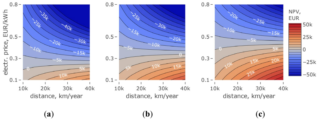
Fig. 3. The NPV as a function of electricity price and yearly distance and for: (a) fuel price = EUR 1 /dm 3 ; (b) fuel price = EUR 1.25 /dm 3 ; (c) fuel price = EUR 1.5 /dm 3 . I_0 = \text{EUR } 2,500
