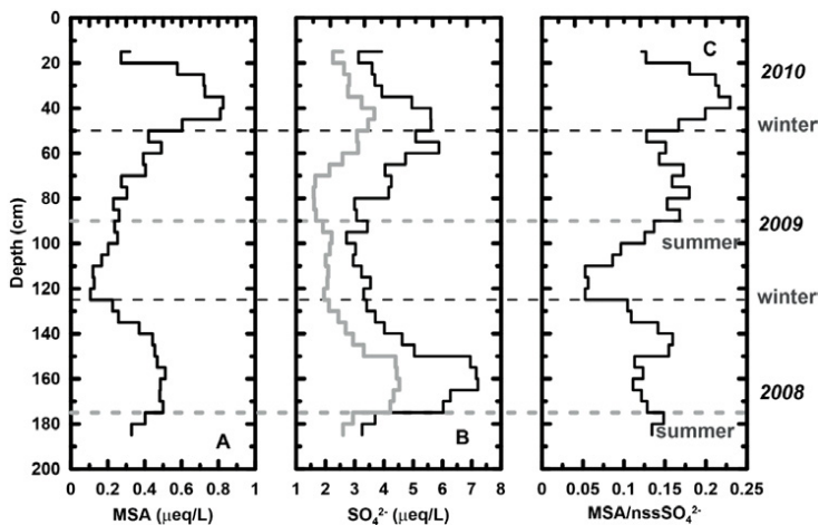
Fig. 5. Vertical profiles of methanesulfonate (MSA) (A), sulfate (B), and MSA/ \text{nssSO}_4^{2-} ratio (C). The gray line in the middle indicates non-sea-salt ( \text{nssSO}_4^{2-} ).
