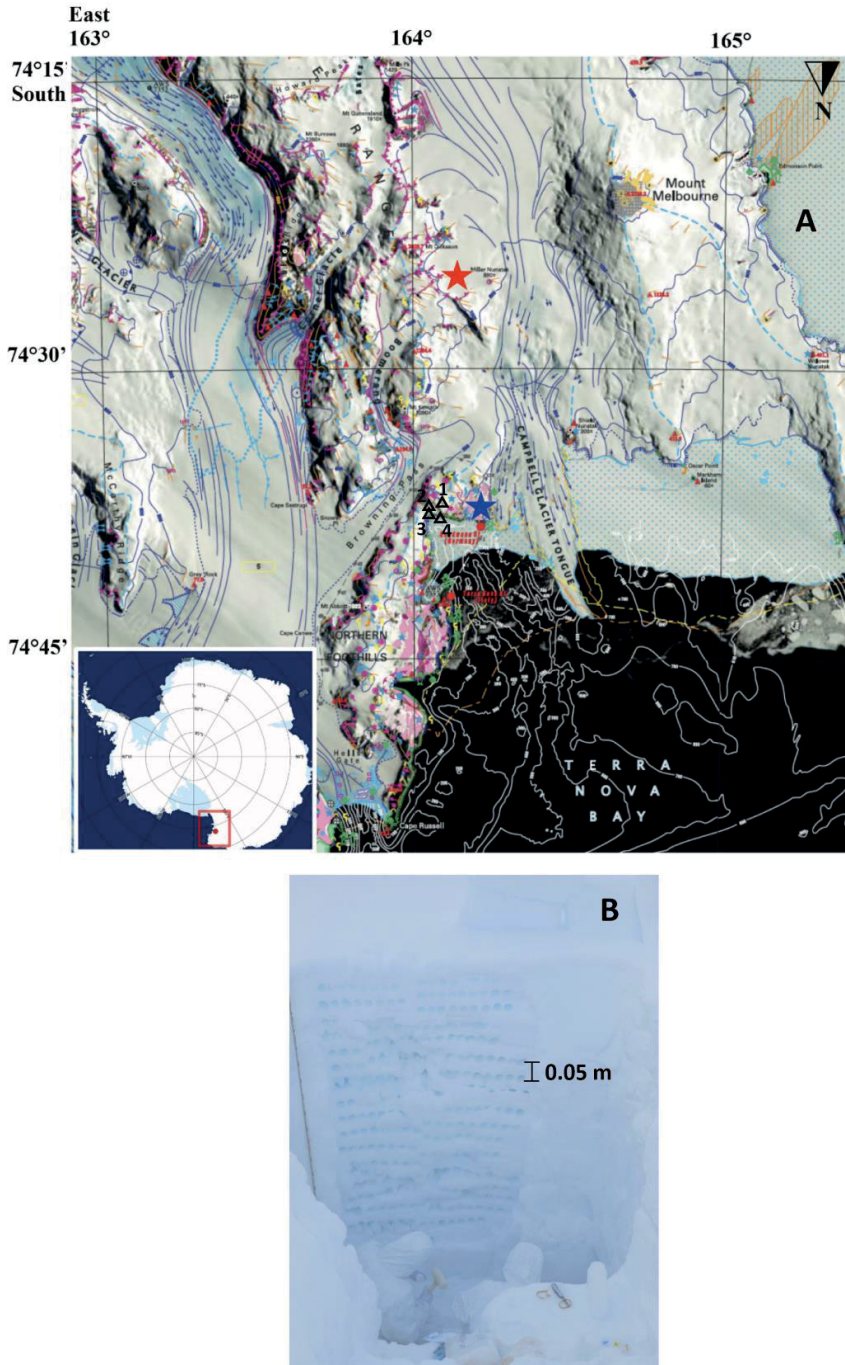
Fig. 1. (A) Location of the snowpit (red star) near the Korean Jang Bogo Station (blue star) in Terra Nova Bay, East Antarctica. Surface snow samples (triangles) are located just near by the station. The surface snow samples were collected before the construction of JBS. The locations of samples were indicated in Table 1. (B) Photo of snowpit.
