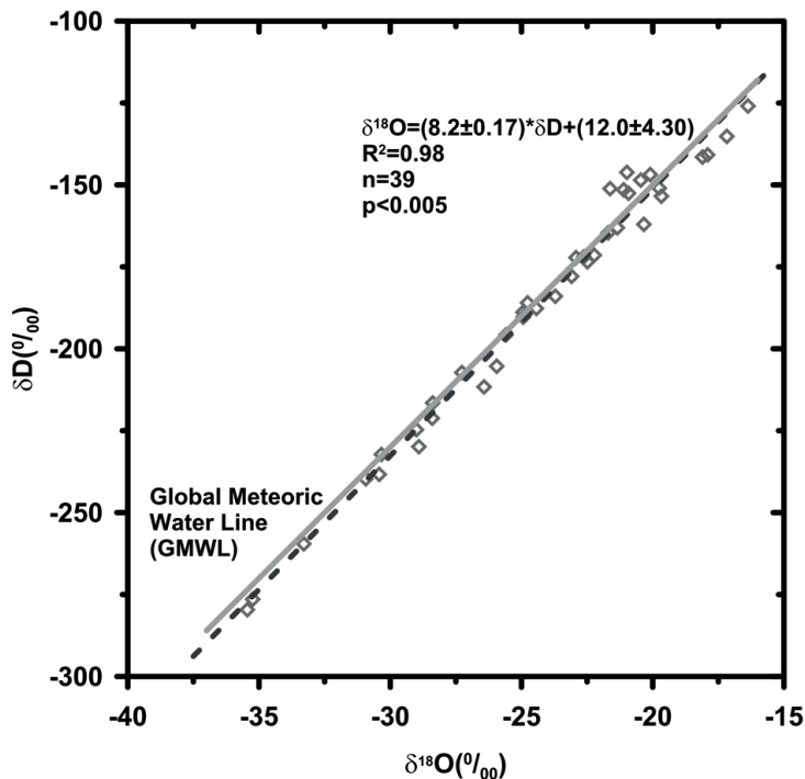
Fig. 2. The linear regression line between \delta\text{D} and \delta^{18}\text{O} . The regression line is similar to that of the GMWL (grey line).
