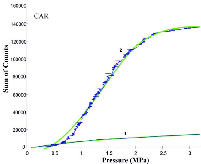
Fig. 4. Sum of counts vs. pressure applied in the direction parallel - 1 or perpendicular - 2 to the bedding plane for a) POL ( d = 660 \text{ mg/cm}^3 ); and b) CAR ( d = 498 \text{ mg/cm}^3 ) composites. Results of measurements - navy-blue curve, polynomial fitting - green line
