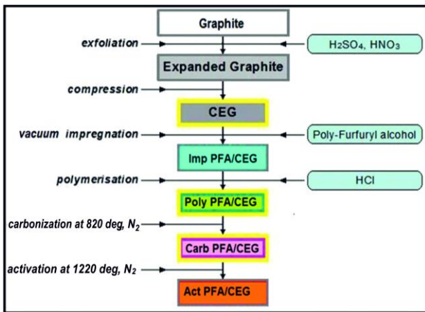
Fig. 1. Schematic diagram of technological procedures of the PFA-polymer/CEG-matrix composites.
