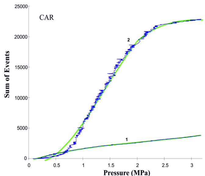
Fig. 5. Dependence of sum of events on pressure applied in the direction parallel - 1 or perpendicular - 2 to the layered structure a) POL ( d = 660 \text{ mg/cm}^3 ); and b) CAR ( d = 498 \text{ mg/cm}^3 ) composites. Results of measurements - navy-blue curve, polynomial fitting - green line
