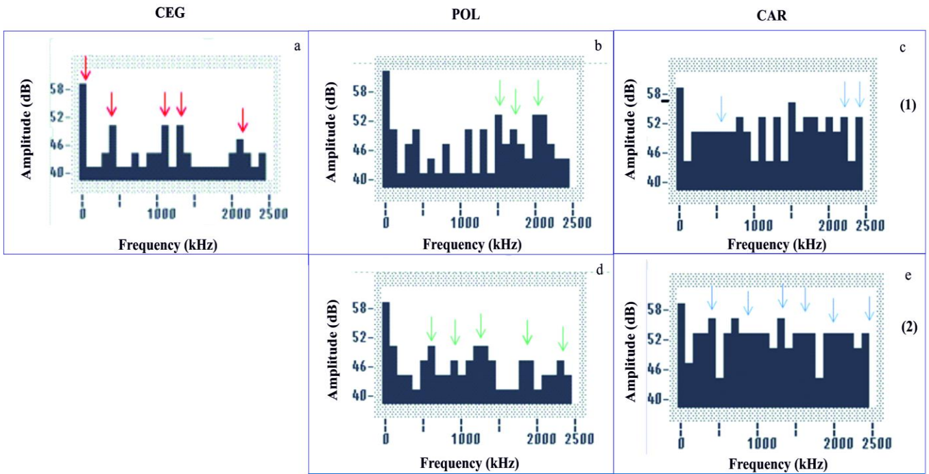
Fig. 8. Fourier analysis of the frequency spectrum of elastic waves for a) CEG d = 107 \text{ mg/cm}^3 ; b) and d) POL d = 660 \text{ mg/cm}^3 ; c) and e) CAR d = 498 \text{ mg/cm}^3 composites, pressure applied in the direction parallel (1) or perpendicular (2) to the layered structure.
