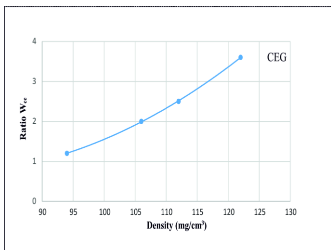
Fig. 6. W_{ce} ratio depending on density of CEG, pressure applied in the direction parallel to layered structure.
