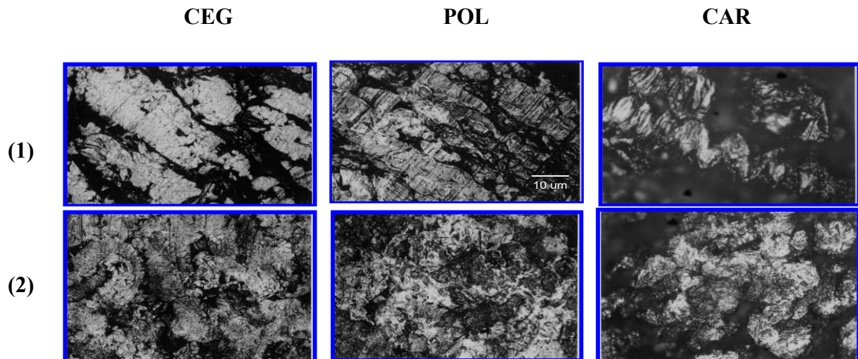
Fig. 2. Microstructures of the composites, (1) - cross-section to the bedding plane, (2) - parallel to the bedding plane a) CEG d = 260 \text{ mg/cm}^3 , b) POL d = 669 \text{ mg/cm}^3 , c) CAR d = 428 \text{ mg/cm}^3 .
