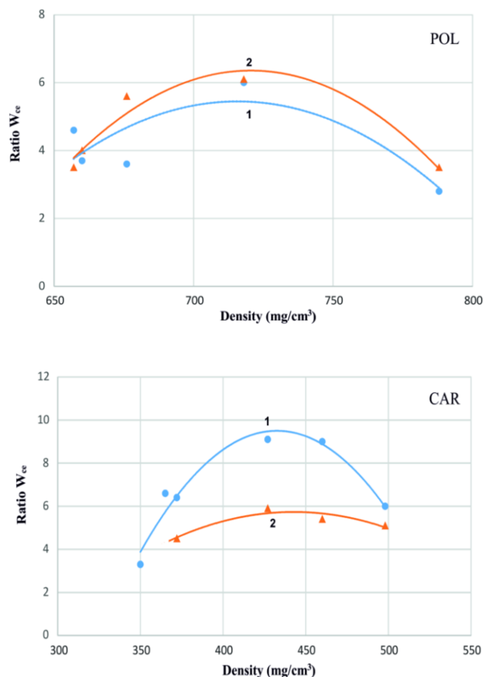
Fig. 7. W_{ce} ratio vs densities of a) POL, b) CAR composite, pressure applied in the direction parallel - 1 or perpendicular - 2 to the bedding plane.
