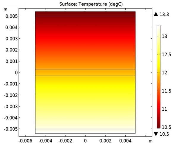
Figure 9: Temperature profile insulating: COMSOL, CO 2 inside skylight.
