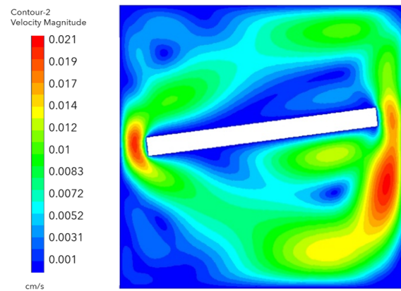
Figure 6: Velocity profile cooling: Fluent, \text{CO}_2 inside skylight.
