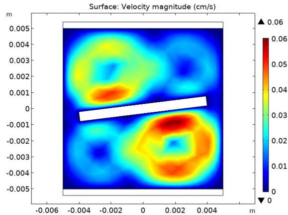
Figure 10: Velocity profile cooling: COMSOL, CO 2 inside skylight.
