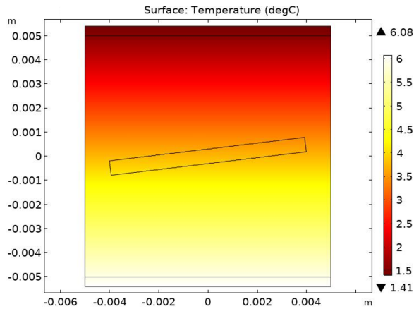
Figure 11: Temperature profile cooling: COMSOL, CO 2 inside skylight.
