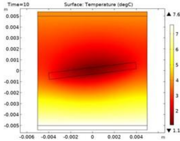
Figure 5: Temperature profile cooling: COMSOL, \text{CO}_2 inside skylight.
