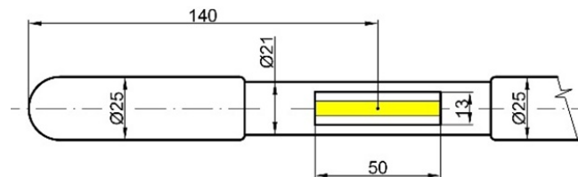
Figure 3: Scheme of optical probe head.
