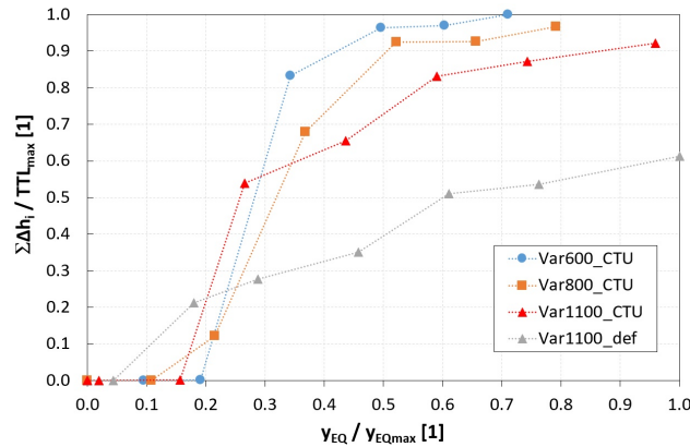
Figure 15: Dependences of normalized total thermodynamic wetness loss (TTL, in kJ/kg) on normalized equilibrium steam wetness.
