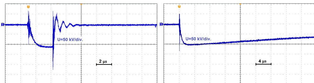
Fig. 6. Example of oscillograms of a voltage waveform: a) when a breakdown occurred, b) when a breakdown did not occur.
