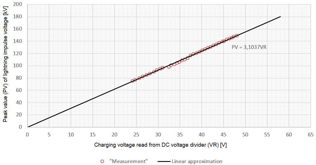
Fig. 5. Generator scaling curve.
