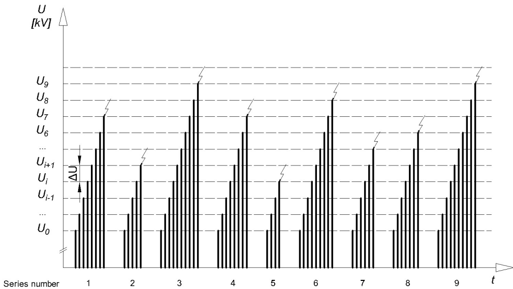
Fig. 2. Example of procedure of an insulation test using the step method.
