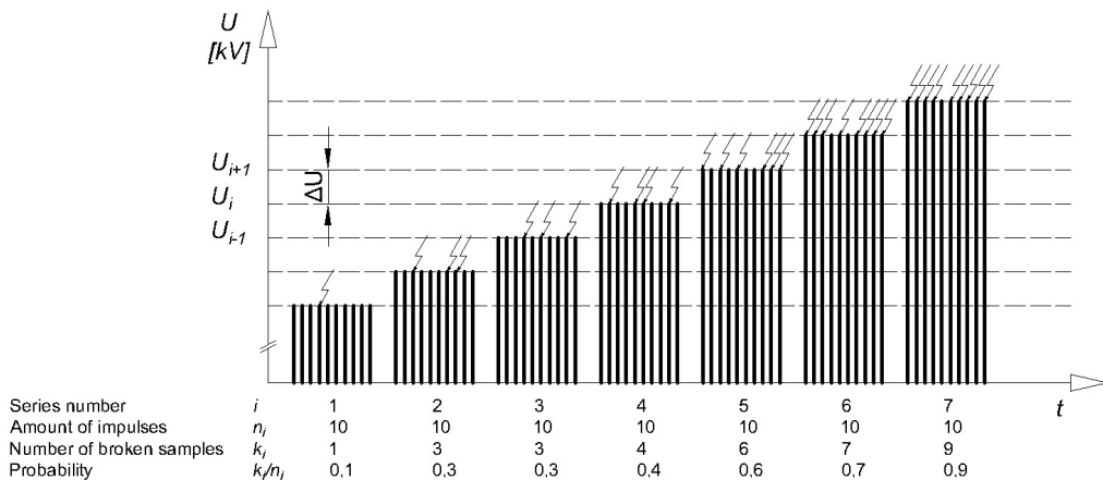
Fig. 1. Example of procedure of an insulation test using the series method.
