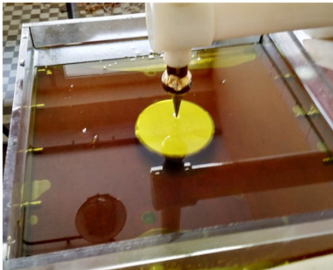
Fig. 4. Real view of the electrode system used in laboratory measurements.
