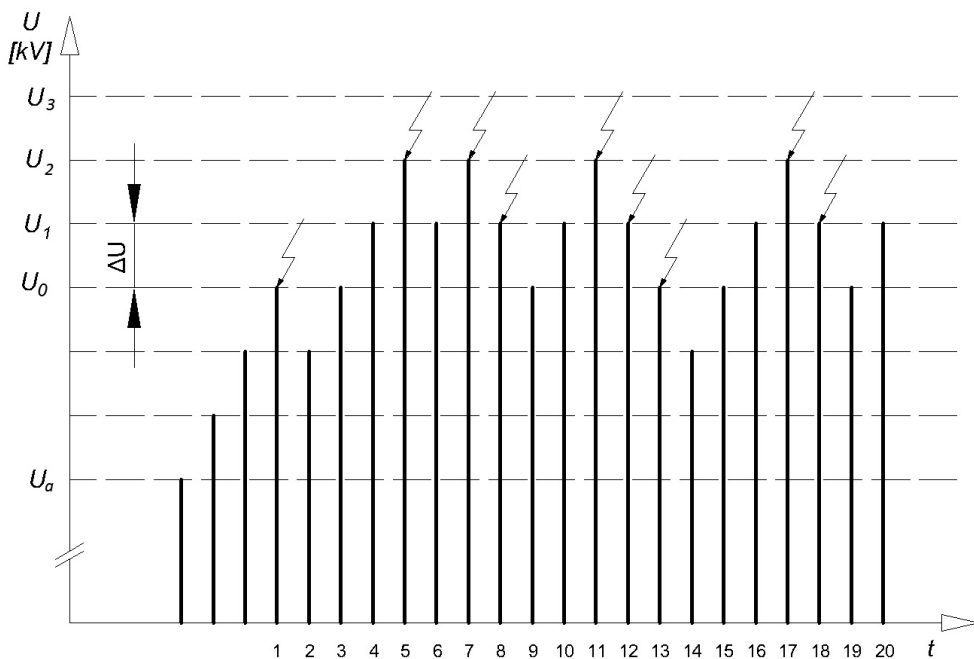
Fig. 3. An example of procedure of an insulation test using the up-and-down method.
