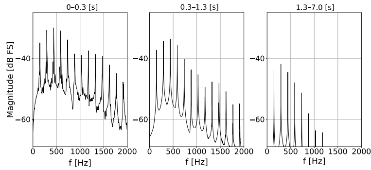
Fig. 8. Averaged spectra recorded for the pitch D3 with the sapele sample.
