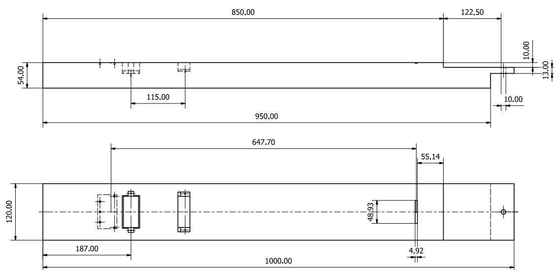
Fig. 1. Schematic drawings of the wood samples used as bases for the simplified electric guitar model.
