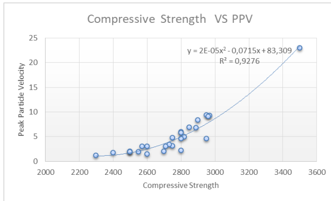
Fig. 15(a). Relation between PPV &amp; Compressive Strength
