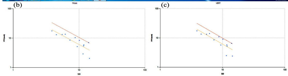
Fig. 12(a-c). Trends of PPV and scaled distance for longitudinal, transverse and vertical in O-PITBLAST
