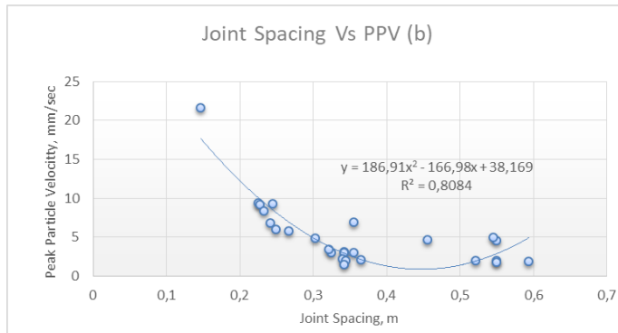
Fig. 15(b). Relation between PPV &amp; Joint Spacing
