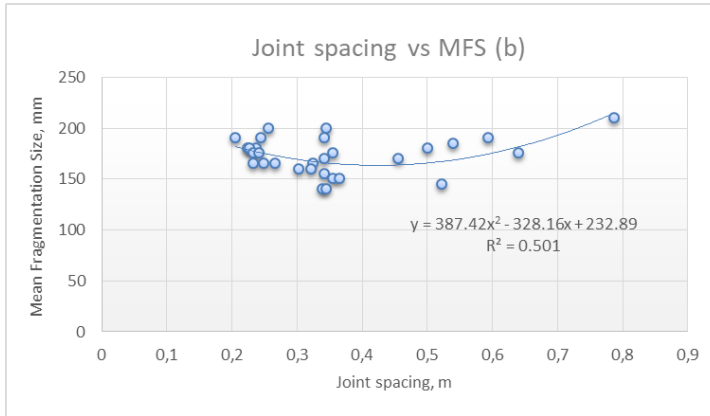
Fig. 14(b). Relation between MFS &amp; Joint Spacing
