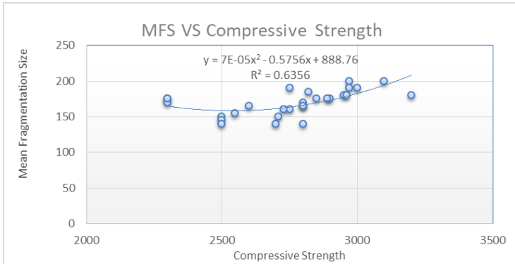
Fig. 14(a). Relation between MFS &amp; Compressive Strength
