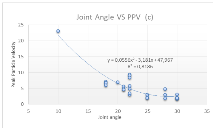
Fig. 15(c). Relation between PPV &amp; Joint angle
