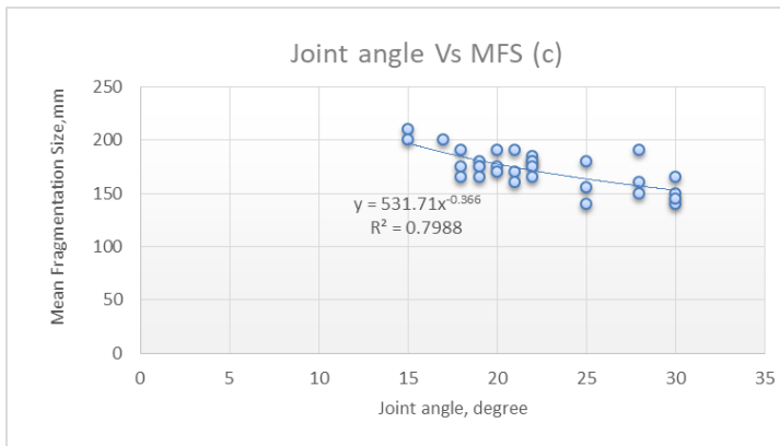
Fig. 14(c). Relation between MFS &amp; Joint angle
