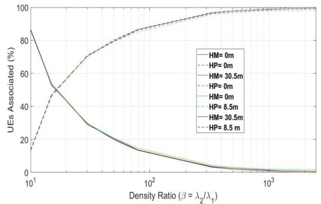
Fig. 3. UEs Association to macro and pico BSs under different two-tier BSs antenna heights Vs BSs density ratio, \beta
