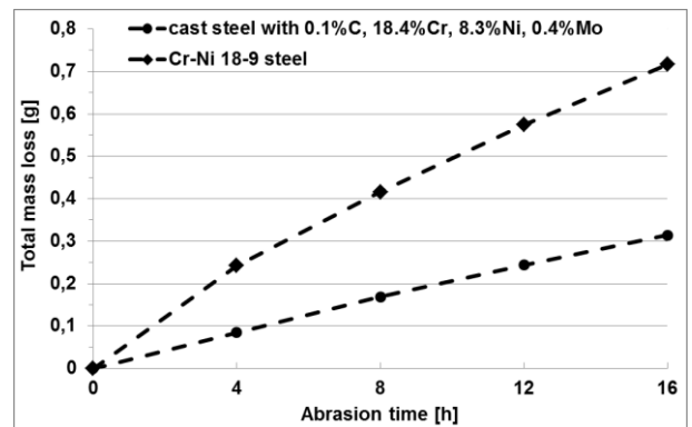
Fig. 3. Mass losses as a function of abrasion time in the Miller test compared for samples made of the Cr-Ni 18-9 steel and cast steel [13]
