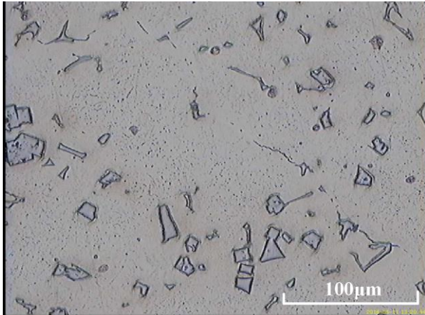
Fig. 4. Microstructure of cast steel with the addition of 2.0% Ti after solution heat treatment; austenitic matrix with primary titanium carbides evenly distributed in this matrix; etched with nital, [11]
