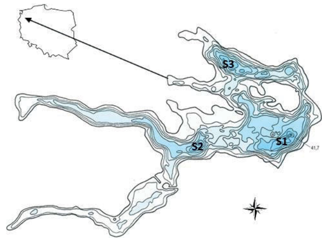
Fig. 1. Location of study sites – Lake Ińsko (53°26'36" N; 15°32'33" E); source: JANCZAK [1996], modified by authors
