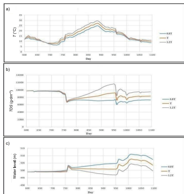
Fig. 8. A diagram of the effect of 20% increase and decrease of air temperature on: a) temperature, b) salinity, c) water level; source: own study
