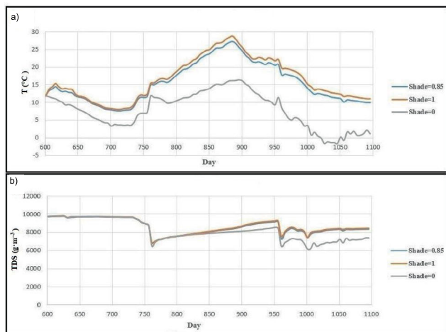
Fig. 7. Changes of: a) temperature ( T ), b) total dissolved solids ( TDS ) for different shade values; source: own study
