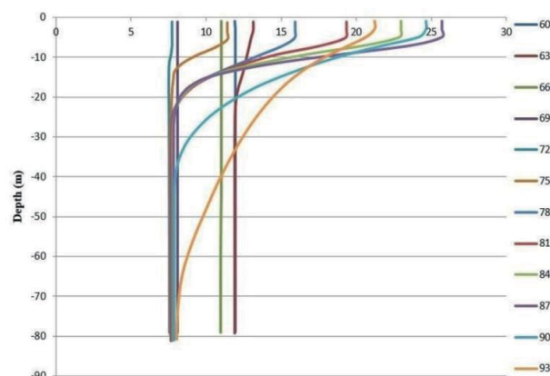
Fig. 4. A diagram of temperature changes in depth; source: own study
