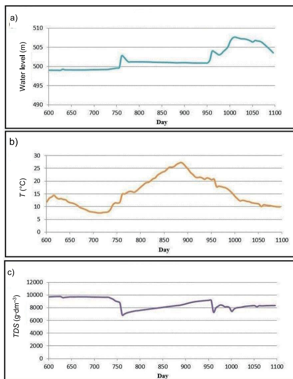
Fig. 3. Diagrams of: a) water level, b) temperature, c) salinity; source: own study
