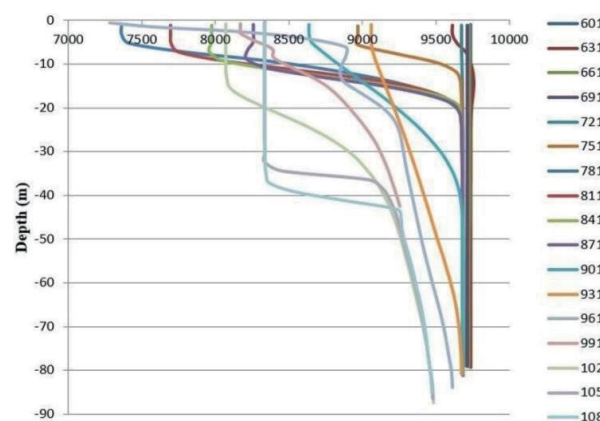
Fig. 5. A diagram of total dissolved solids ( TDS ) changes in depth; source: own study
