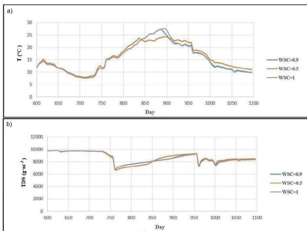
Fig. 6. Changes of: a) temperature ( T ), b) total dissolved solids ( TDS ) for different values of wind shear coefficient ( WSC ); source: own study
