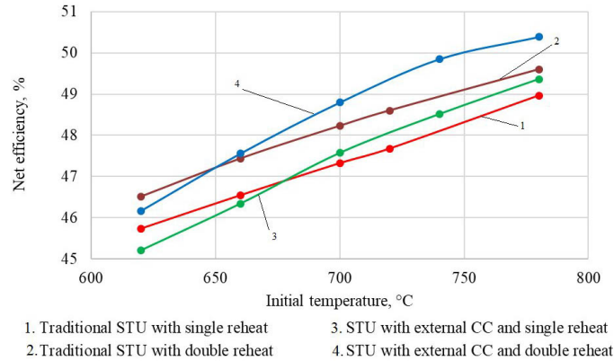
Figure 8: Initial temperature influence on the net efficiency of steam turbine power plants with different types of reheat.
