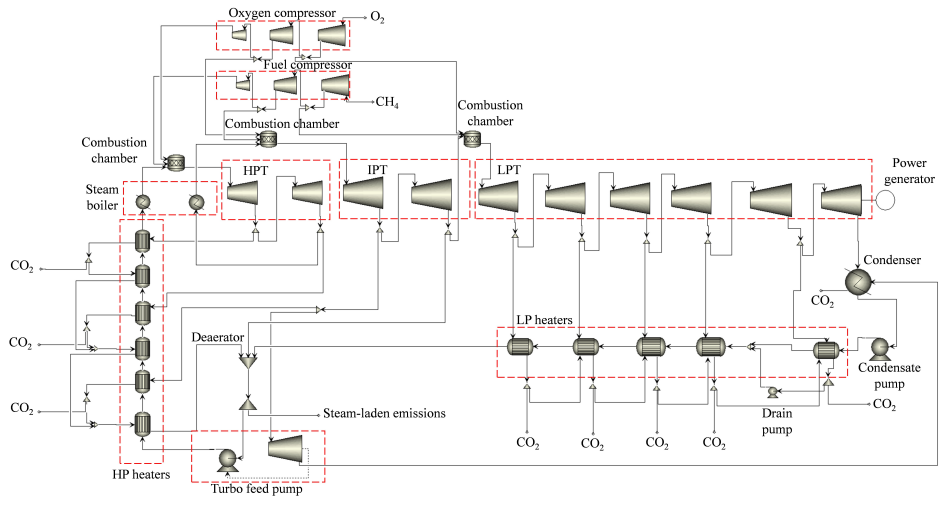
(b) double reheat
