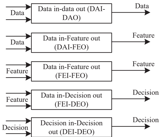
Fig. 2. Dasarathy's classification
