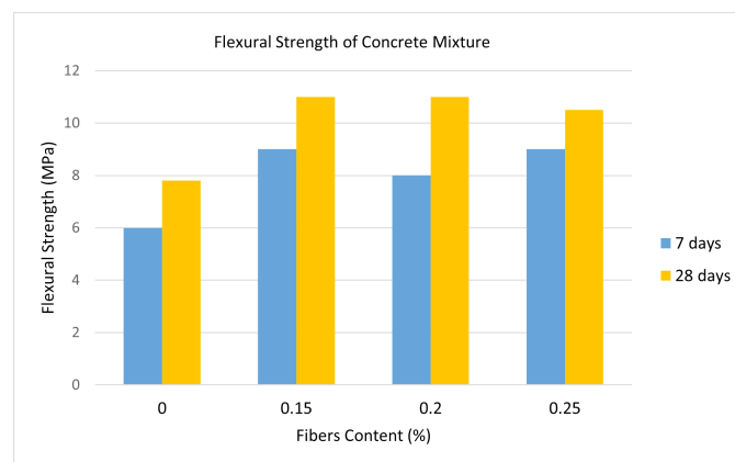
Fig. 3. The flexural strength of fiber reinforced geopolymer concrete [30]
