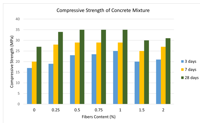
Fig. 2. Compressive strength versus fibers content [49]
