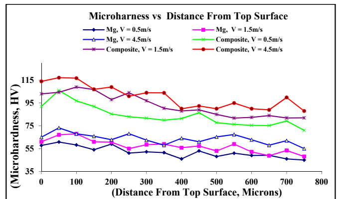
Fig. 13. Variation of microhardness of the wear tested specimens of pure Mg and surface composite at 12 N load
