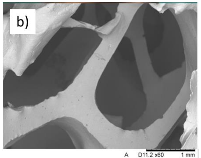
Fig. 2. Open-porous cast Al-Si12 foam: a) sample during compression test, b) SEM micrograph – general view
