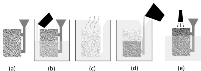
Fig. 1. Scheme of the investment casting process of metallic foams
