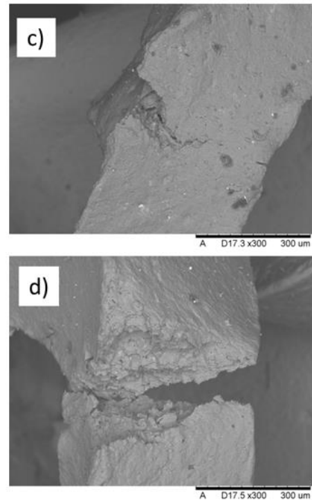
Fig. 4. View of the samples after compression tests: a), b) general view with marked damage types, c) crack initiation, d) brittle fracture
