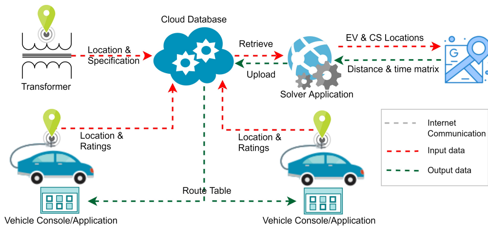
Fig. 2. Architecture
