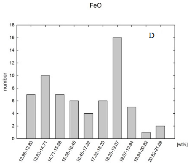
Fig. 13D. Histogram of FeO content in allanites
