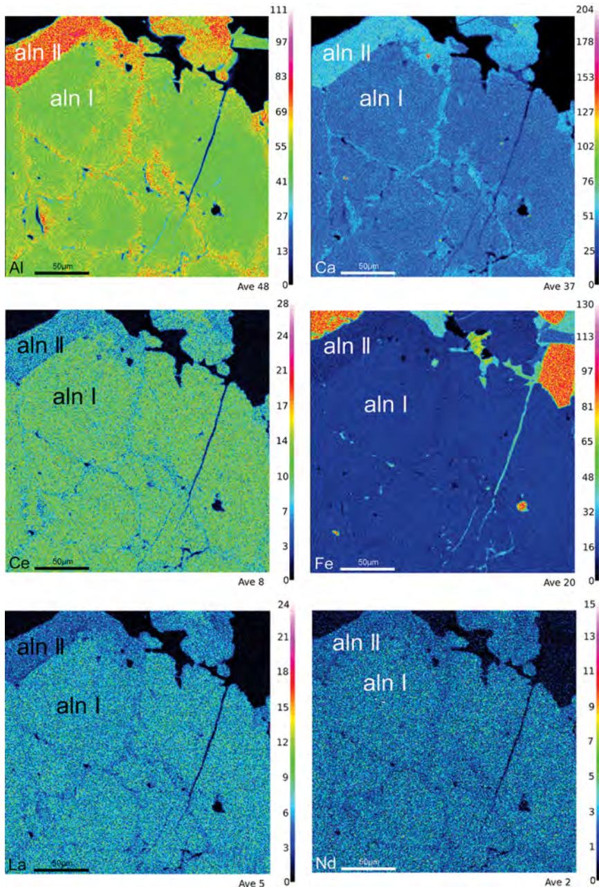
Fig. 7. WDS compositional maps of two allanite populations Al – contour map of Al, Ca contour map of – Ca, Ce contour map of – Ce, Fe contour map of – Fe, La contour map of – La, and Nd contour map of – Nd (revised from Hao et al. 2021)
