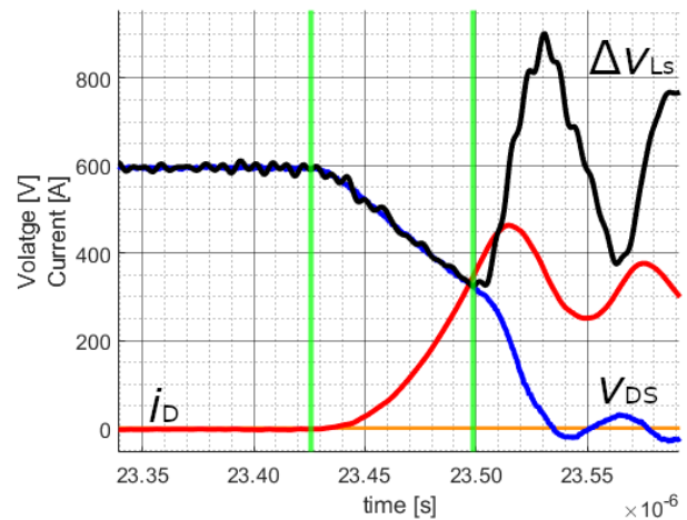
Fig. 6. Proper time alignment of voltage and current waveforms
