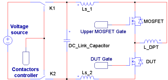
Fig. 1. Simplified schematic of the double-pulse test testbench
